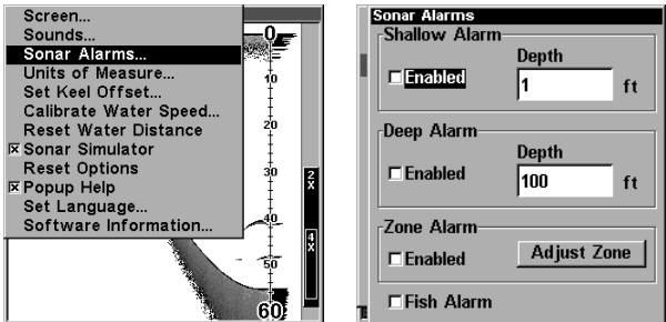
At left, Main Menu and Sonar Alarms command. At right, the Sonar Alarms menu.
