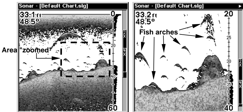
Normal display, in auto depth range mode, left. At right, display "zoomed" with Upper and Lower Limits focusing on the portion of the water column from 20 feet to 40 feet deep. In the "zoomed" image, note the target definition at lower left, showing a fish holding just above the structure. At top right, two game fish are attacking a school of bait fish.
