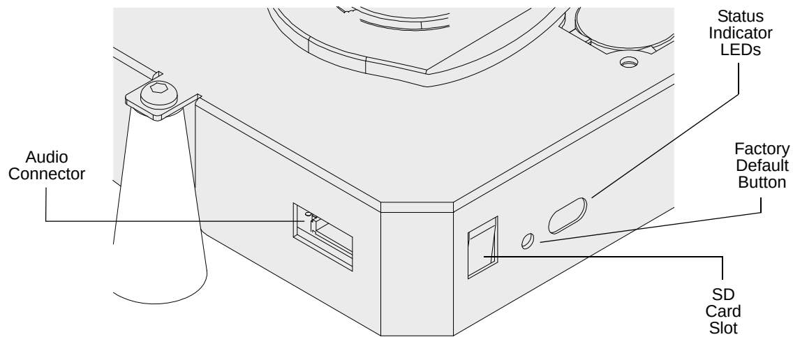
Fig. 2: Camera Connections
