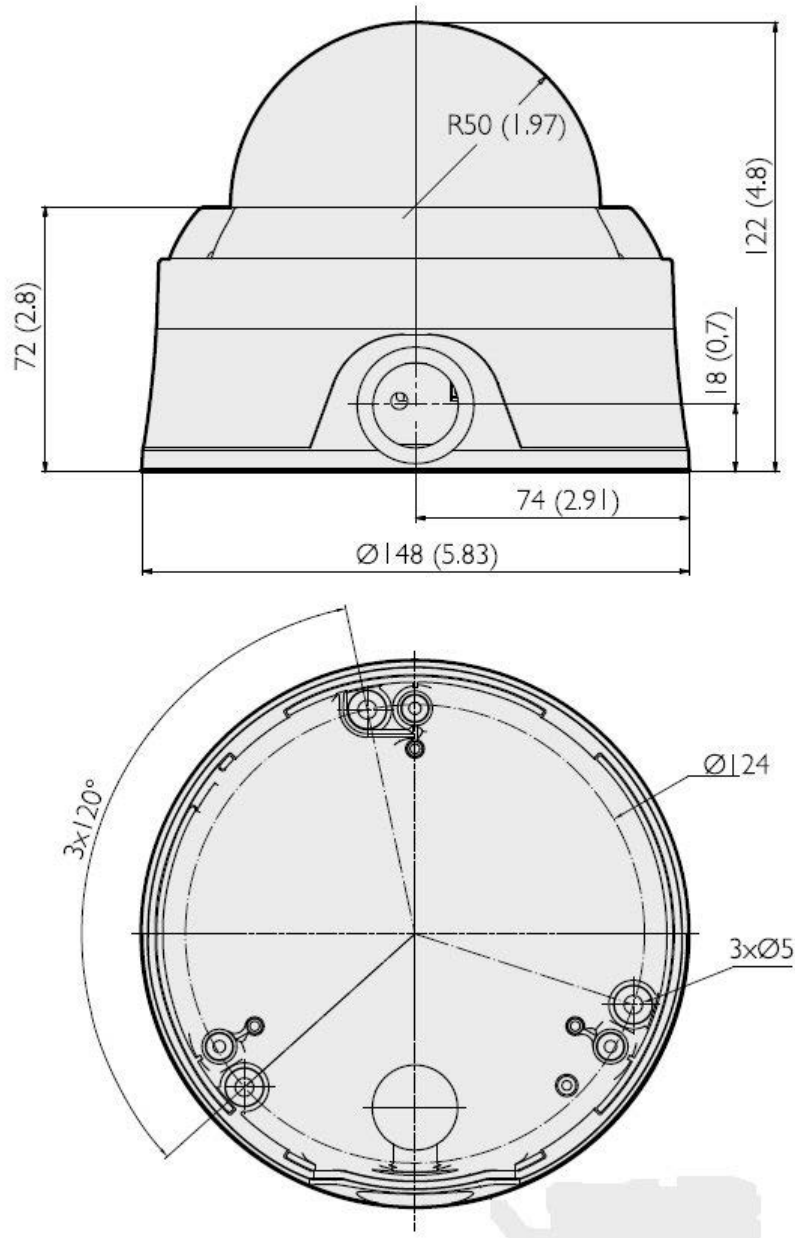
Fig. 20: Dimensions in mm (inches)
