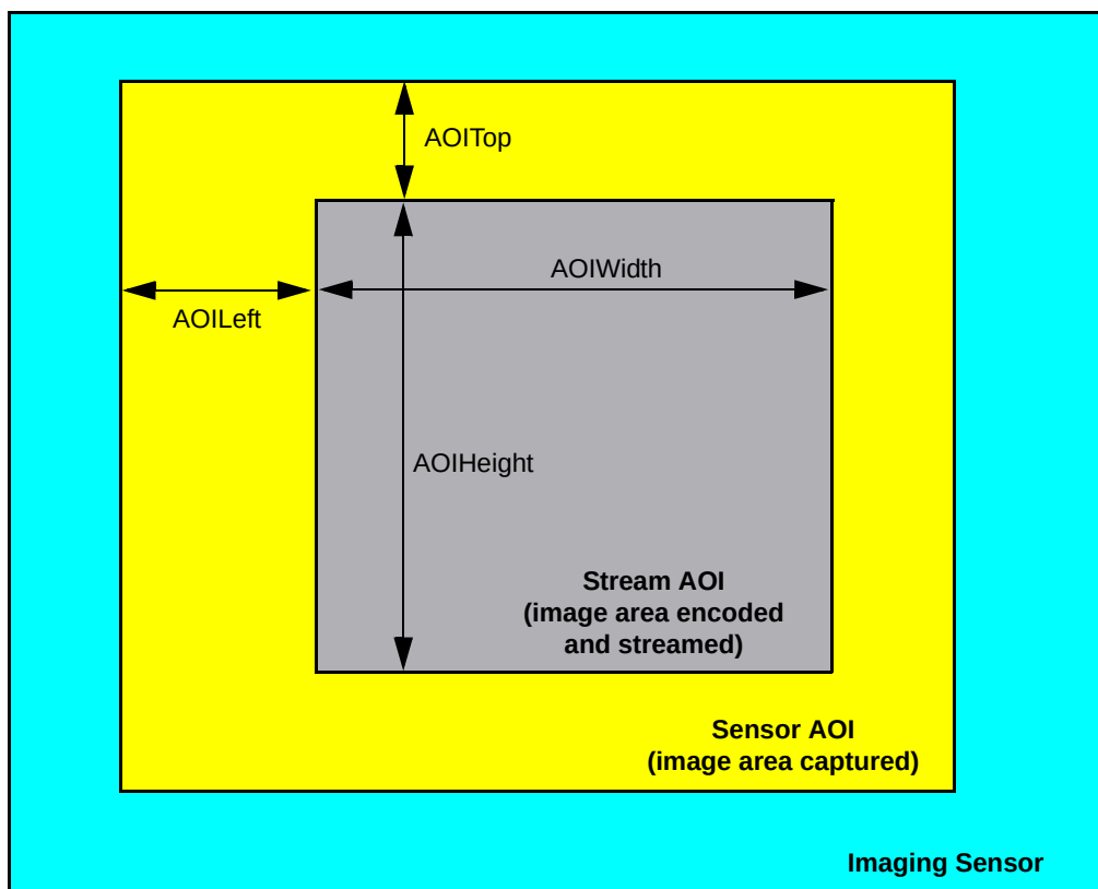
Fig. 5: Stream AOI
