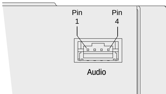
Fig. 13: Audio Connector
