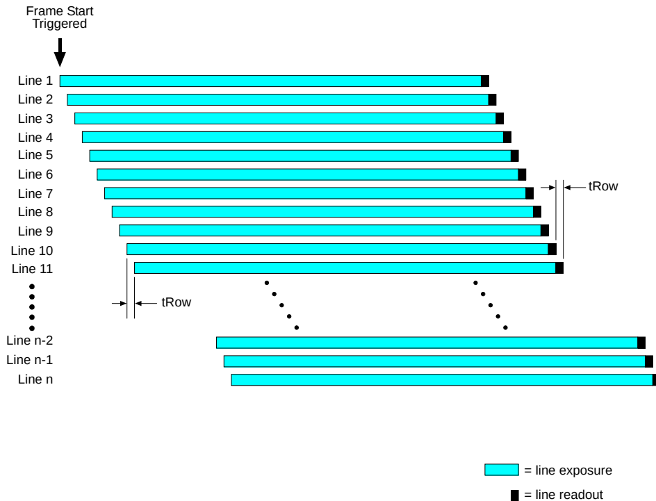
Fig. 6: Rolling Shutter
