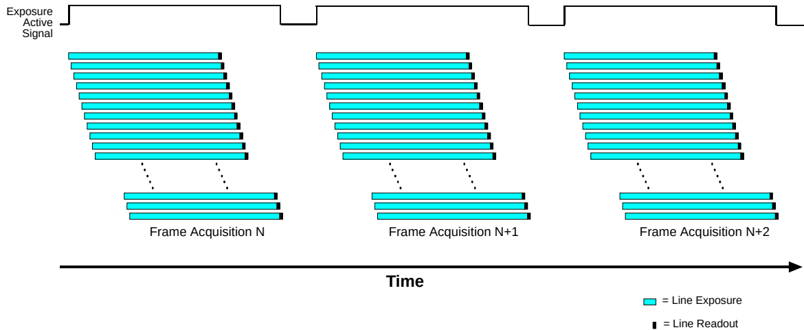
Fig. 9: Exposure Active Signal
