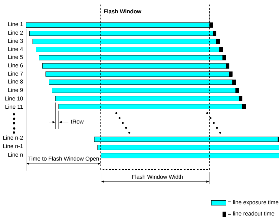
Fig. 7: Flash Window
