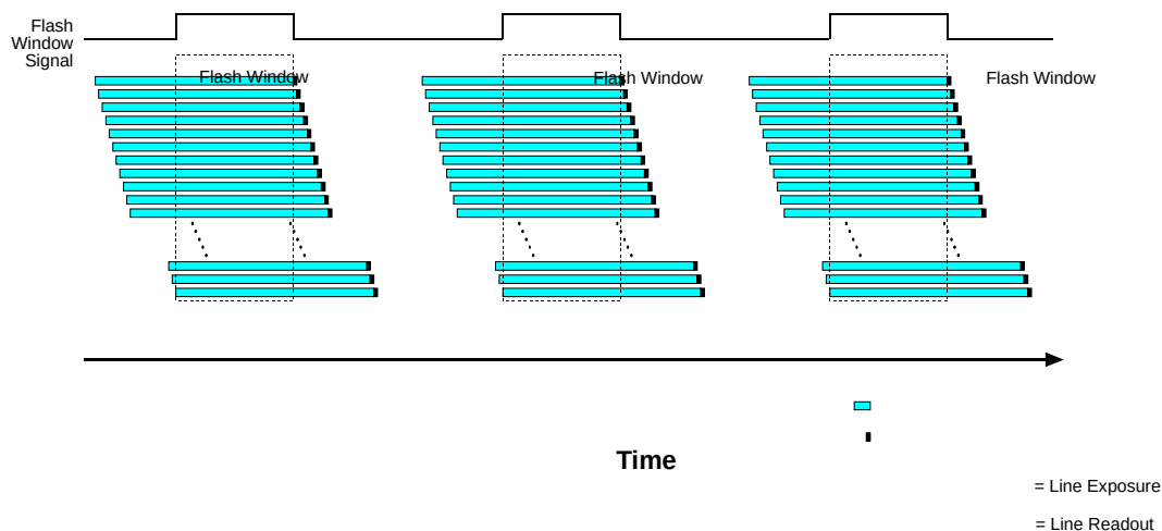
Fig. 8: Flash Window Signal
