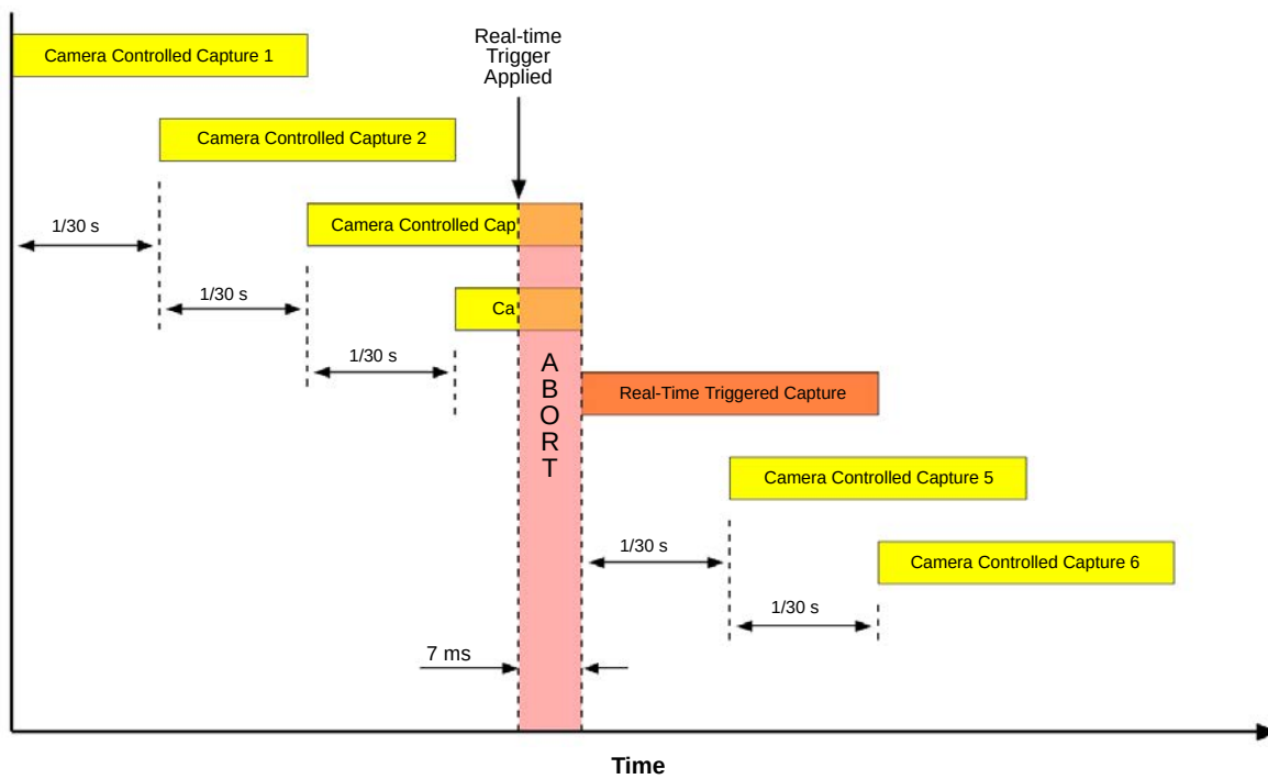
Fig. 19: Real-Time Trigger Image Capture
