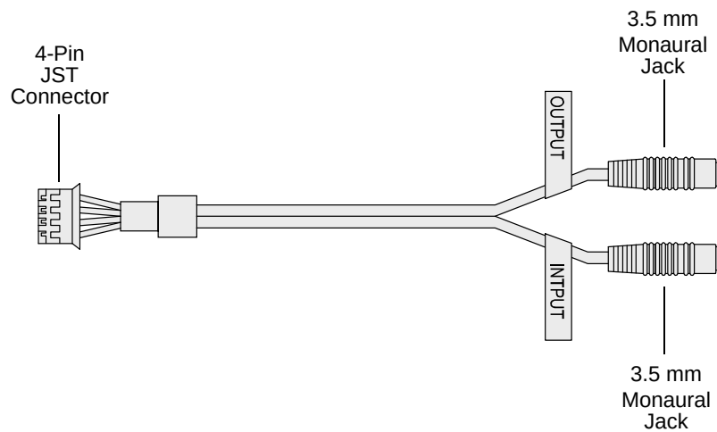
Fig. 14: Audio Y-Cable
