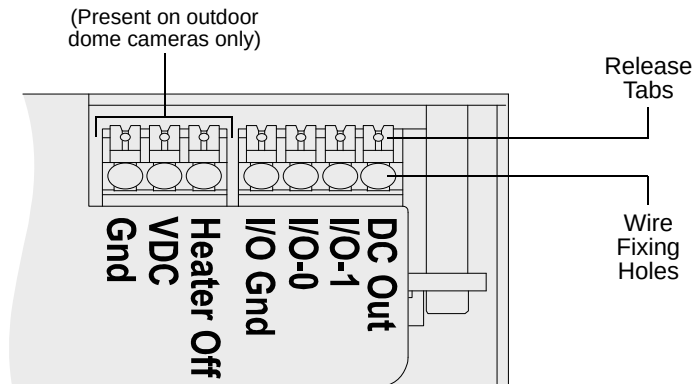
Fig. 10: Main Terminal Block
