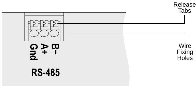
Fig. 12: RS-485 Terminal Block
