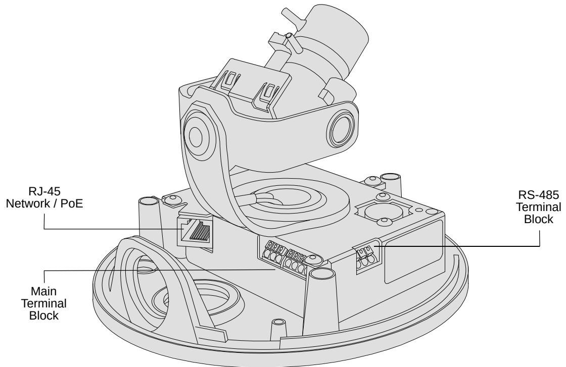
Fig. 1: Camera Connections
