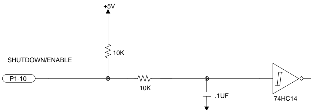
Figure 1-5. Enable/Shutdown Inputs
