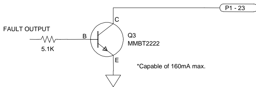
Figure 1-4. Fault Output
