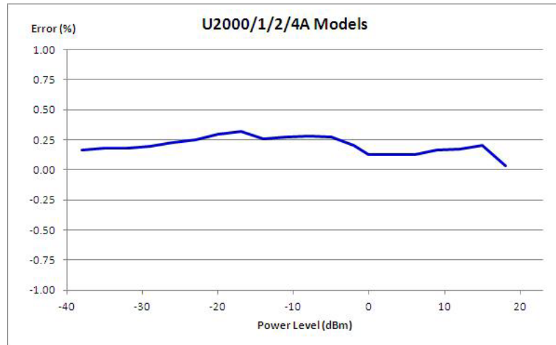
Figure 3-10 Typical power accuracy at 25 °C for U2000/1/2/4A models 1, 2
