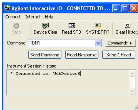
Figure 1-10 Agilent Interactive IO dialog box
