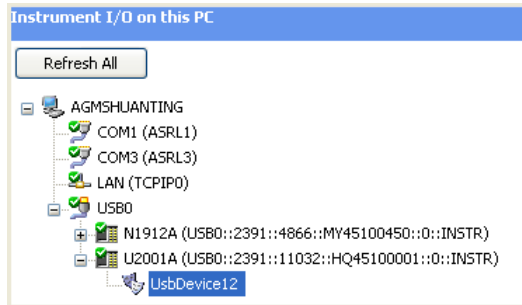
Figure 1-9 Agilent Connection Expert with a list of instrument I/O on the PC
