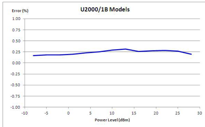
Figure 3-11 Typical power accuracy at 25 °C for U2000/1B models 1, 2
