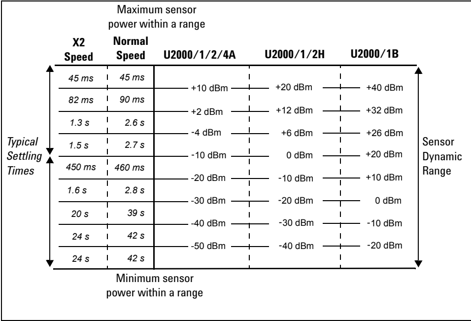
Figure 3-13 Settling time with auto filter, default resolution, and a 10 dB decreasing power step (not across the switching point)
