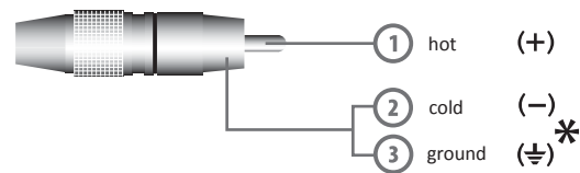
2TRK IN, OUT lack (unbalanced)
