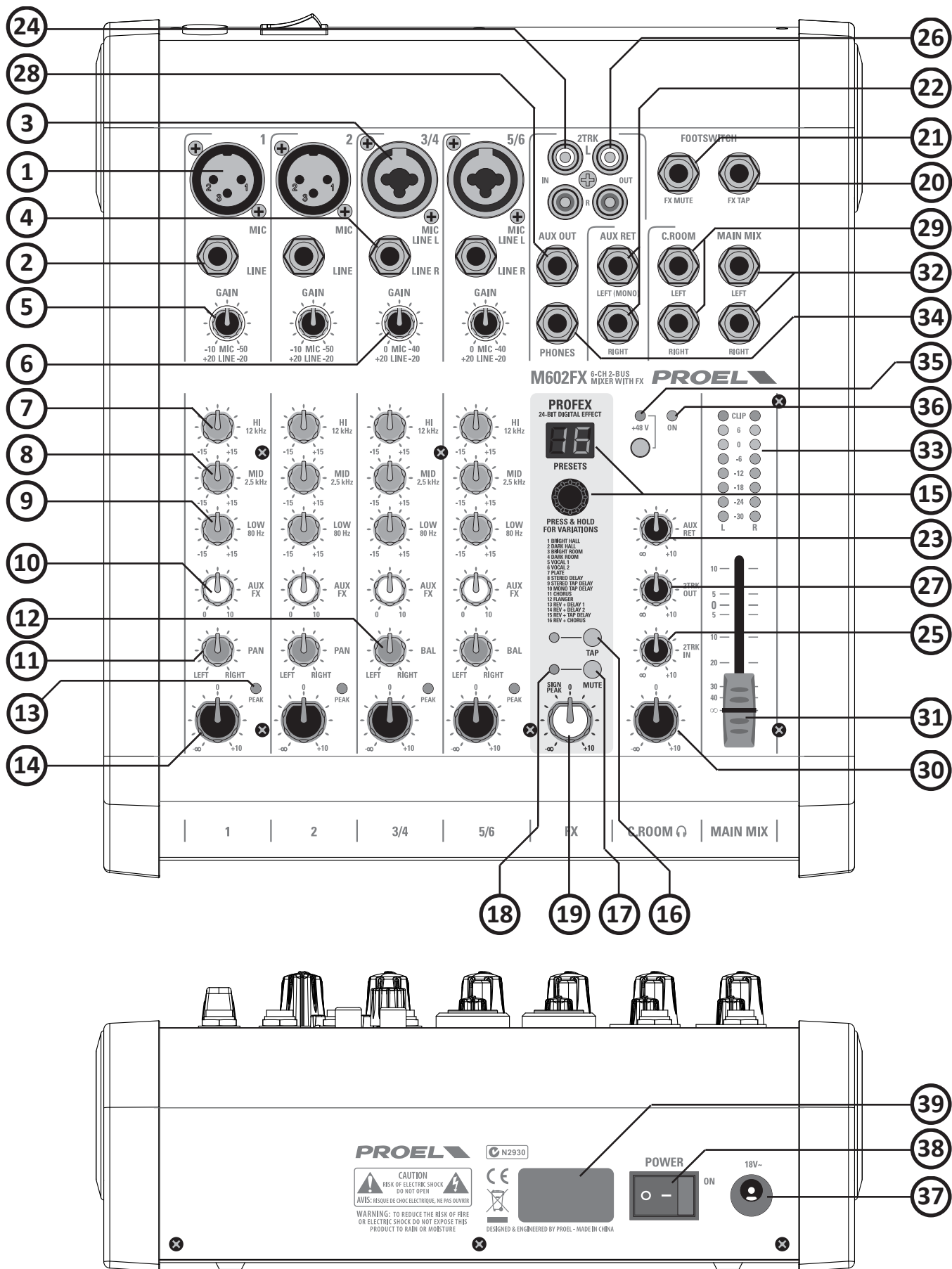
CONTROL PANEL (FIG.2)
