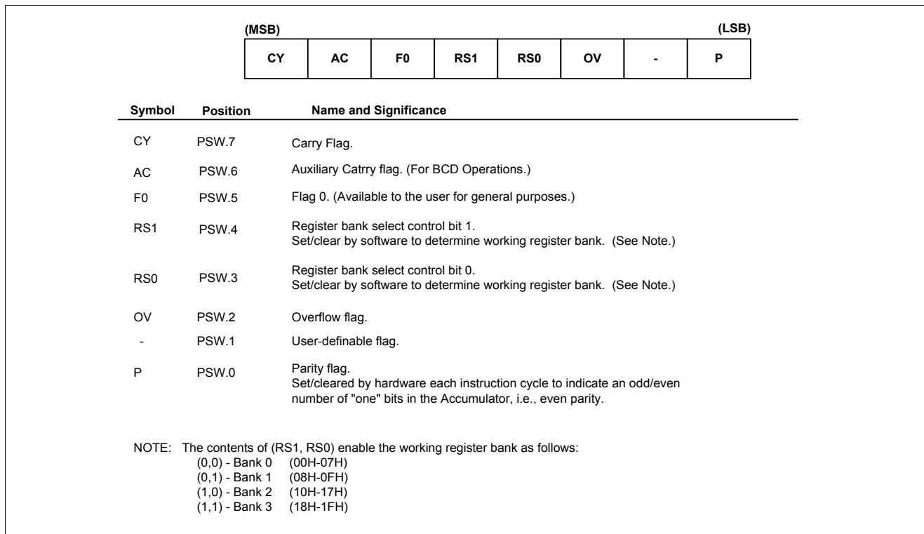
Figure 4-1 Program Status Word (PSW) Register
