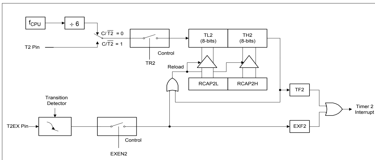
Figure 3-11 Timer 2 in Auto-Reload Mode
