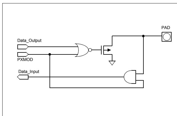
Figure 3-30 P2.0, P2.1, P2.2 and P2.3 Ports Schematic
