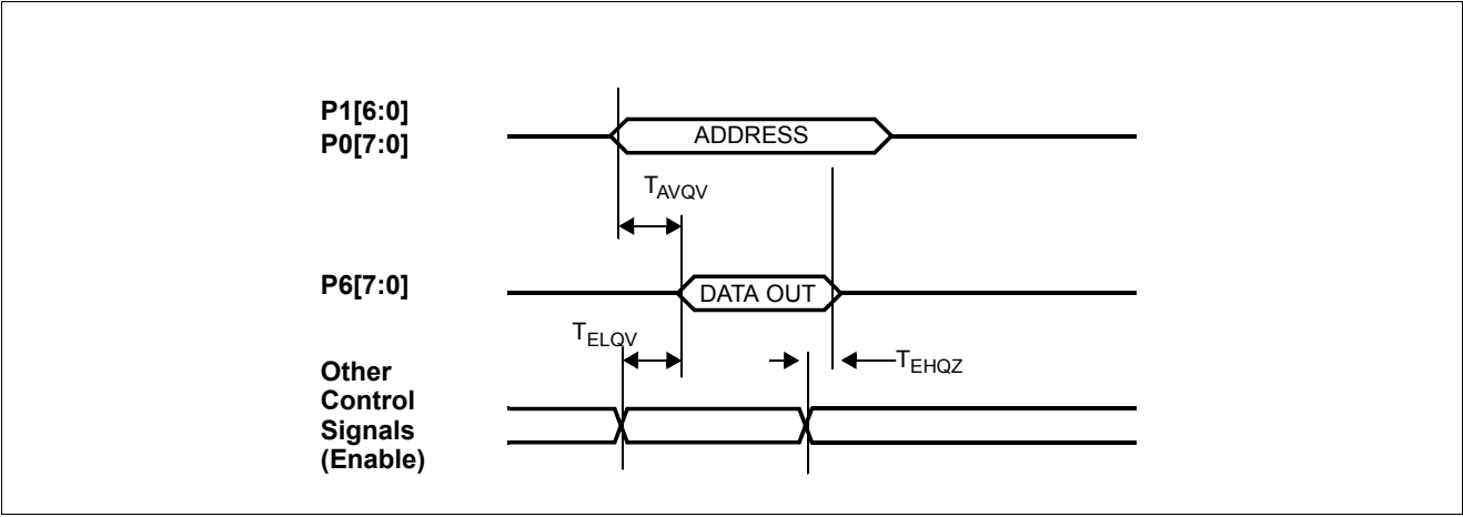
Figure 7-5 Two Consecutive Read Waveform
