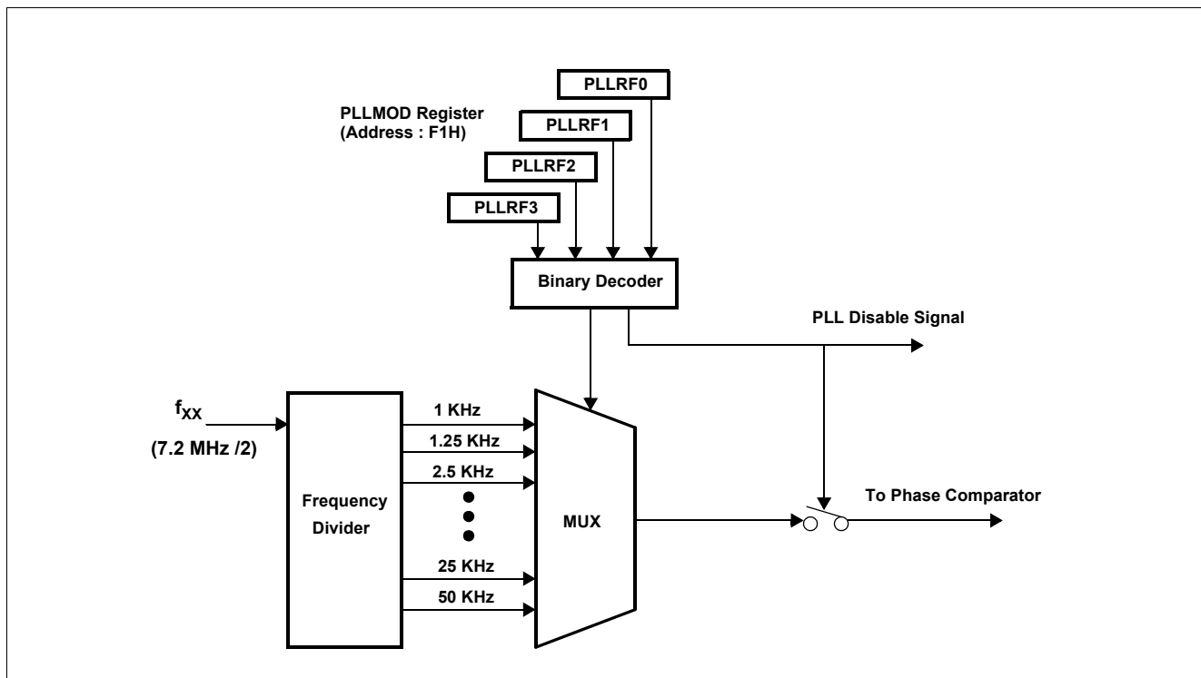
Figure 3-40 Reference Frequency Generator Configuration
