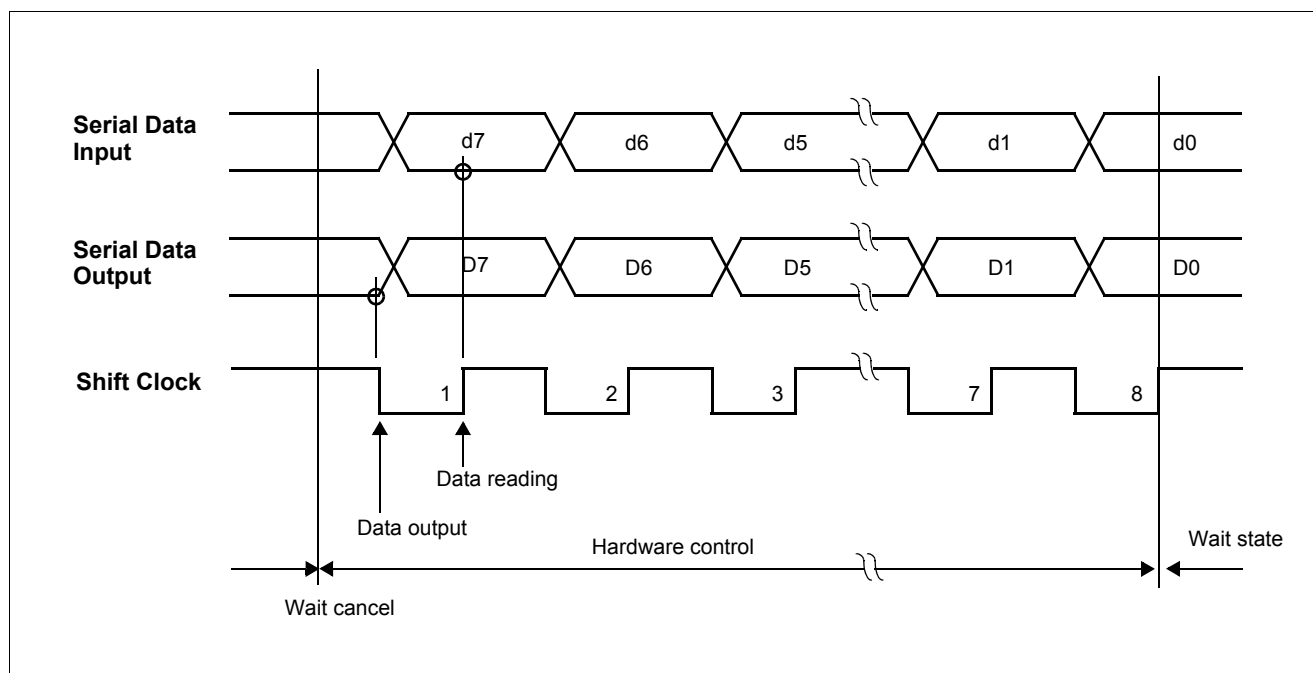
Figure 3-27 Input/Output Block of the SIO and Communication Method
