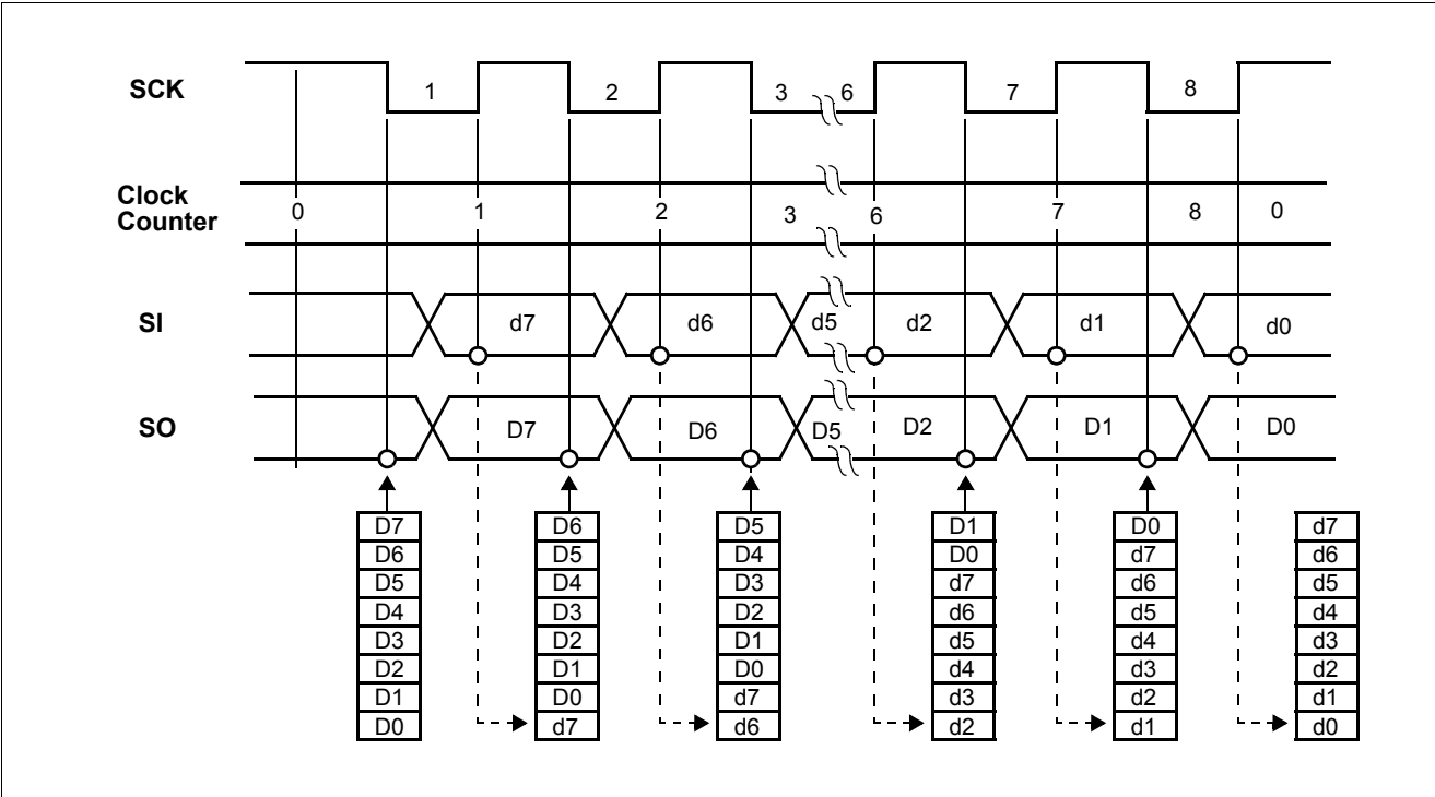
Figure 3-25 SIO1 and SIO2 Timing Diragram
