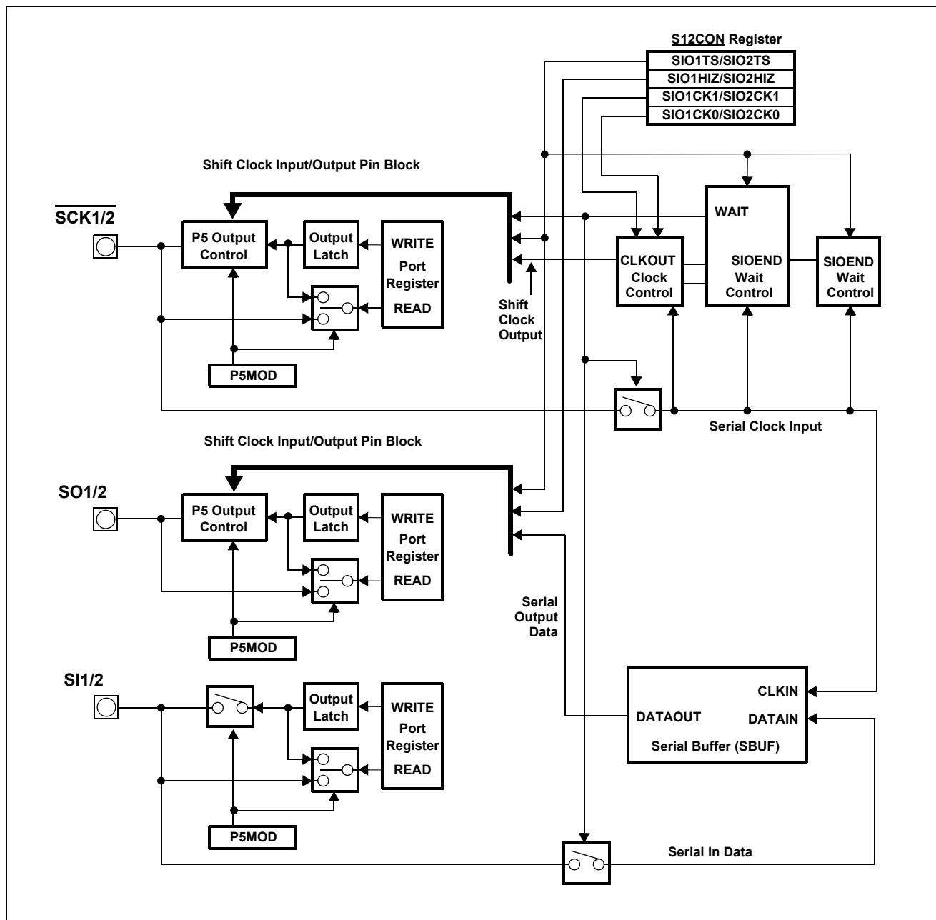
Figure 3-22 SIO Block Diagram
