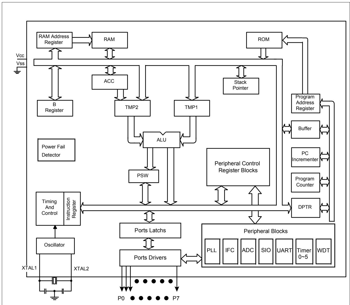
Figure 3-1 HMS9XC8132 Architecture
