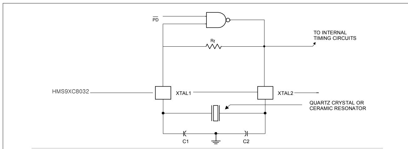
Figure 3-52 Using the CMOS On-Chip Oscillator
