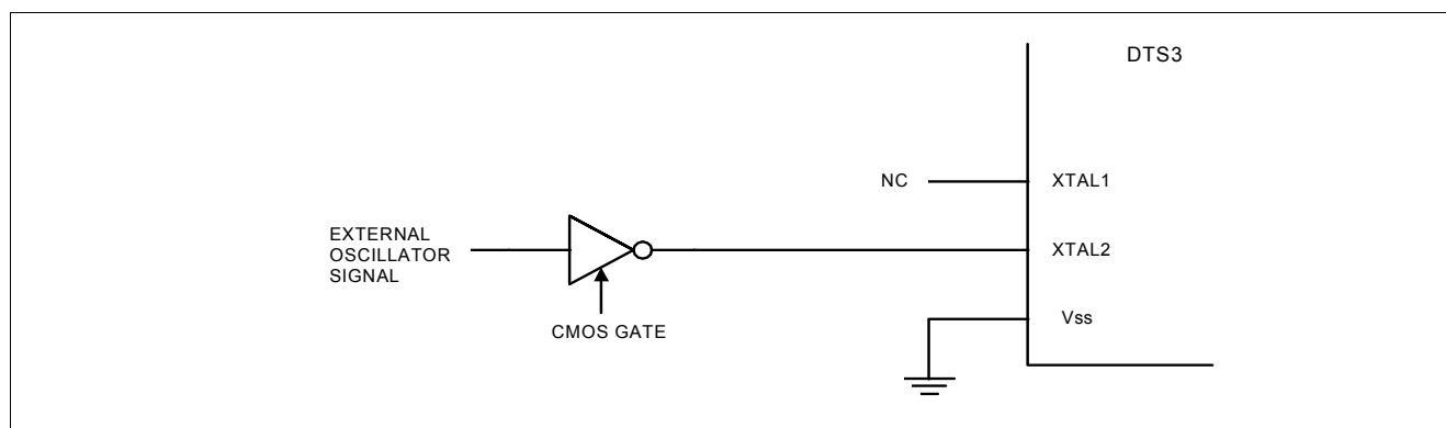
Figure 3-53 Driving the CMOS Family Parts with an External Clock Source
