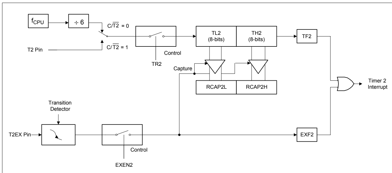
Figure 3-10 Timer2 in Capture Mode
