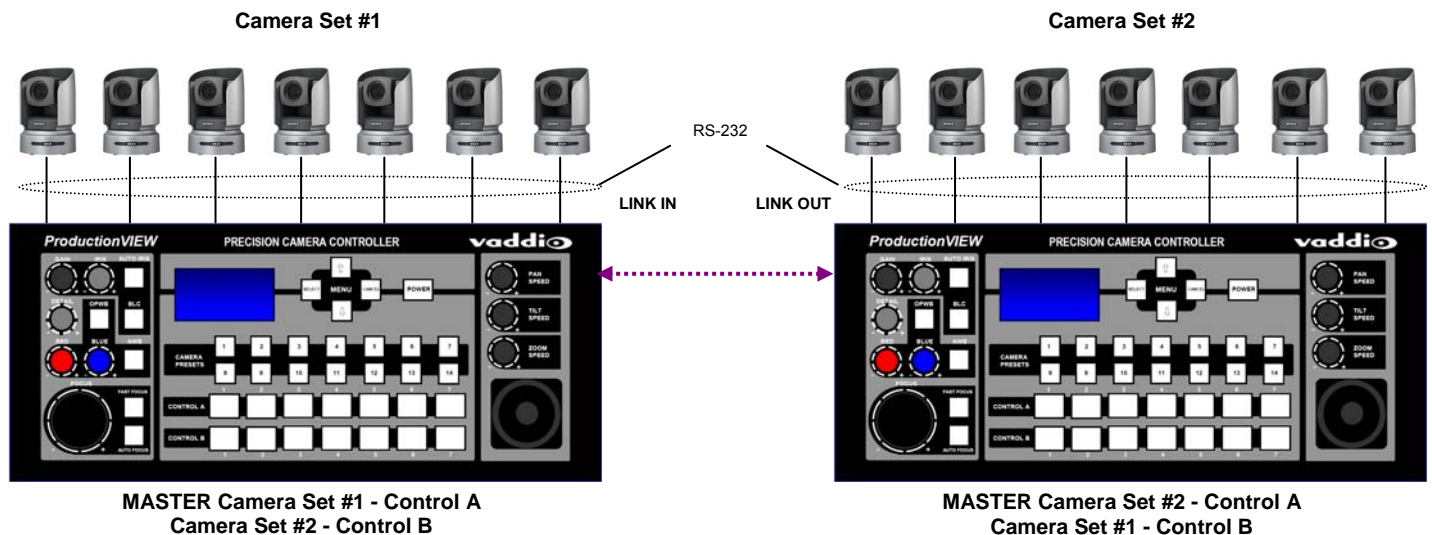
Figure 7: Two Precision Camera Controllers set up in Link Mode. Each Precision Camera Controller has 7 cameras connected, and all cameras can be controlled from either Precision Camera Controller, however not concurrently. There can be two operators, but only one operator can access all fourteen cameras at any point in time. As an example, both the Master and the Secondary can operate their own Control A bus cameras concurrently, but in order for the Master to control the B bus of the Secondary Precision Camera Controller, then operator at the Secondary position must remain idle. An external switcher may not be connected to Precision Camera Controller in Dual Link mode. Both Precision Camera Controllers must be set to Control A under the Camera Select Bus menu.
