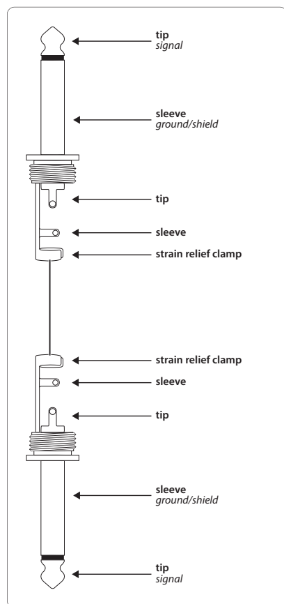
Fig. 9.1: Unbalanced 1/4" cable with 1/4" TS plugs
