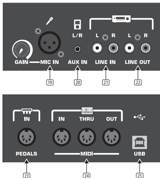
Fig. 3.2: Connectors of the EG2280USB/EG8280USB
