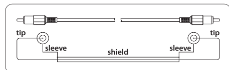
Fig. 9.2: Hi-fi RCA cable
