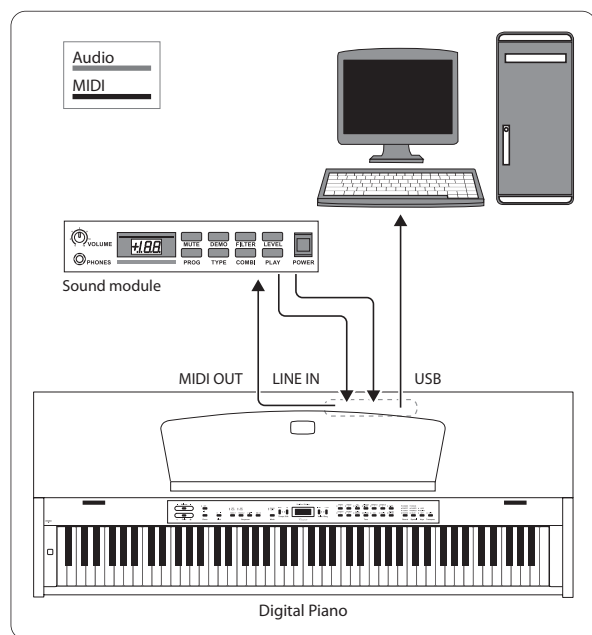
Fig. 6.4: USB connection with an external sound module.
