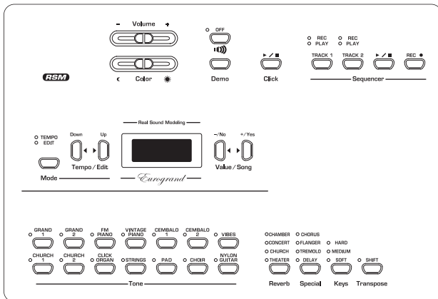
Fig. 3.1: Control elements of the EG2280USB/EG8280USB
