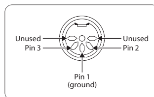
Fig. 9.4: MIDI plug pin assignment
