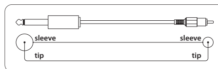
Fig. 9.3: 1/4" to RCA cable
