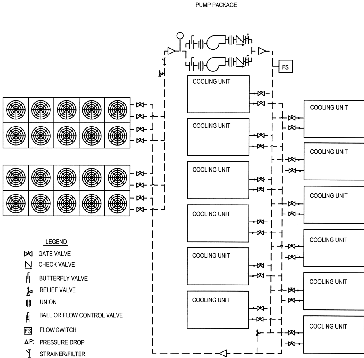
Figure 1 Typical application
