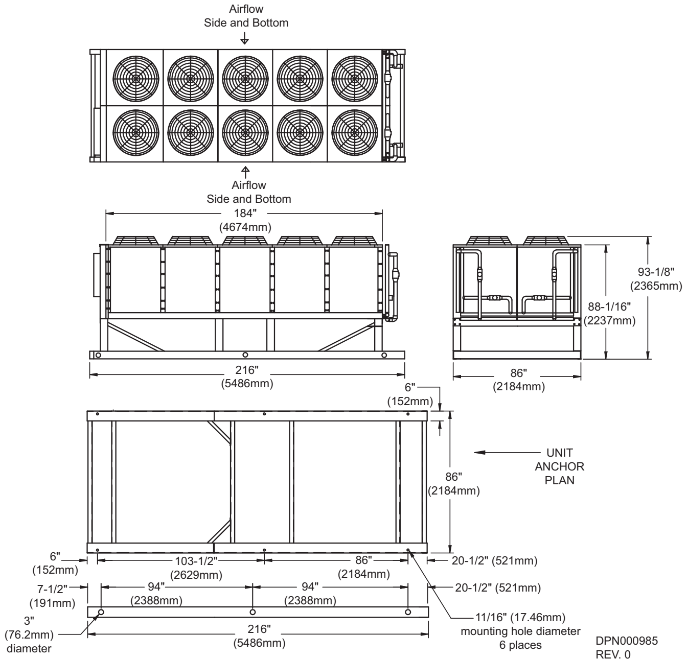
Figure 5 Unit dimensions
