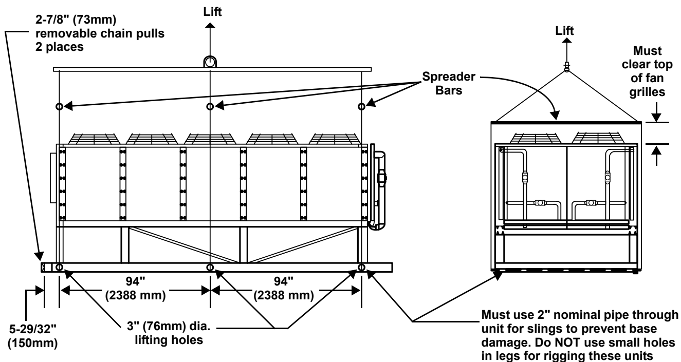
Figure 6 Rigging instructions
