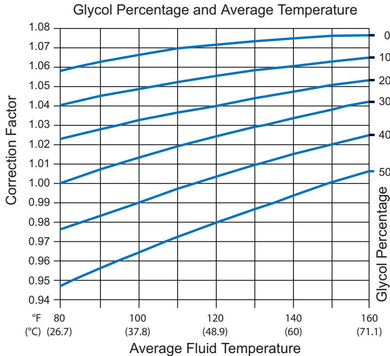
Figure 2 Capacity correction factor
