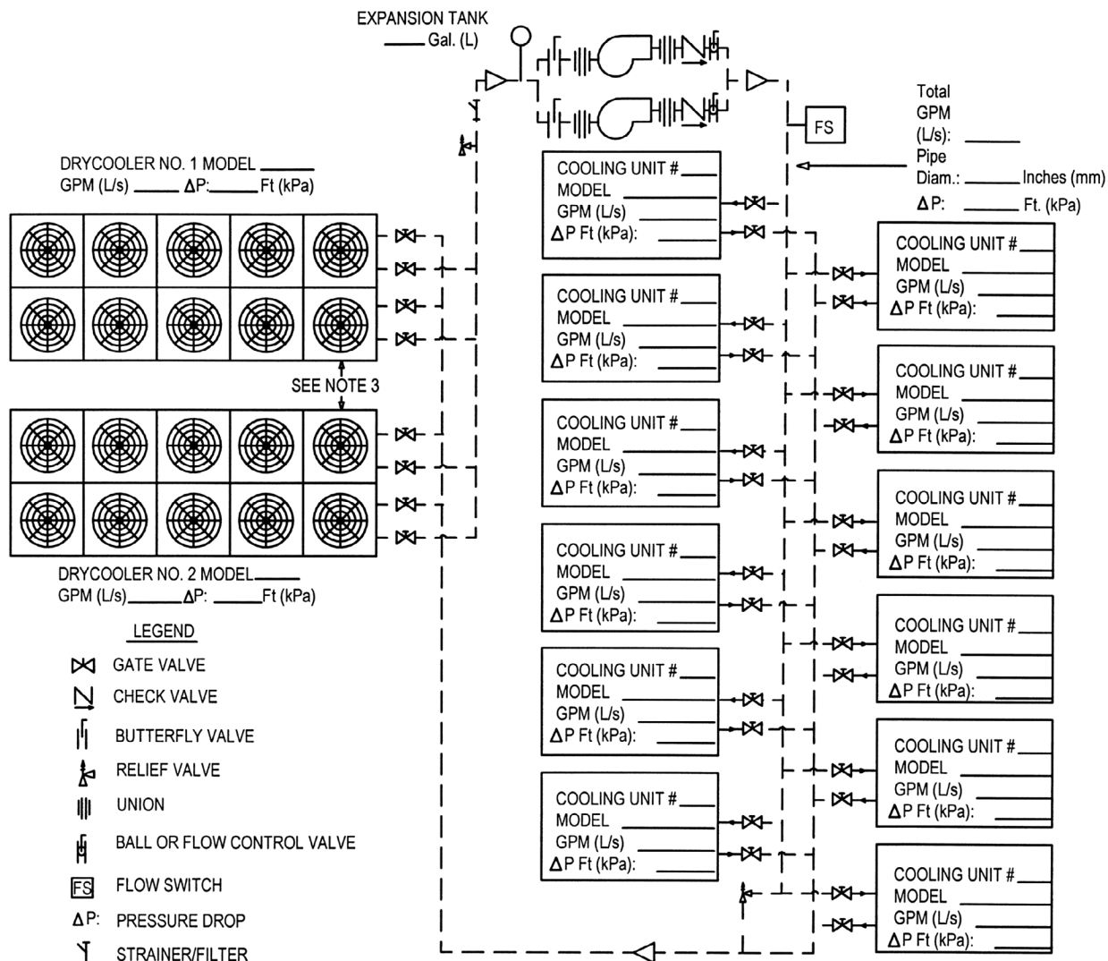
Figure 7 Typical piping diagram
