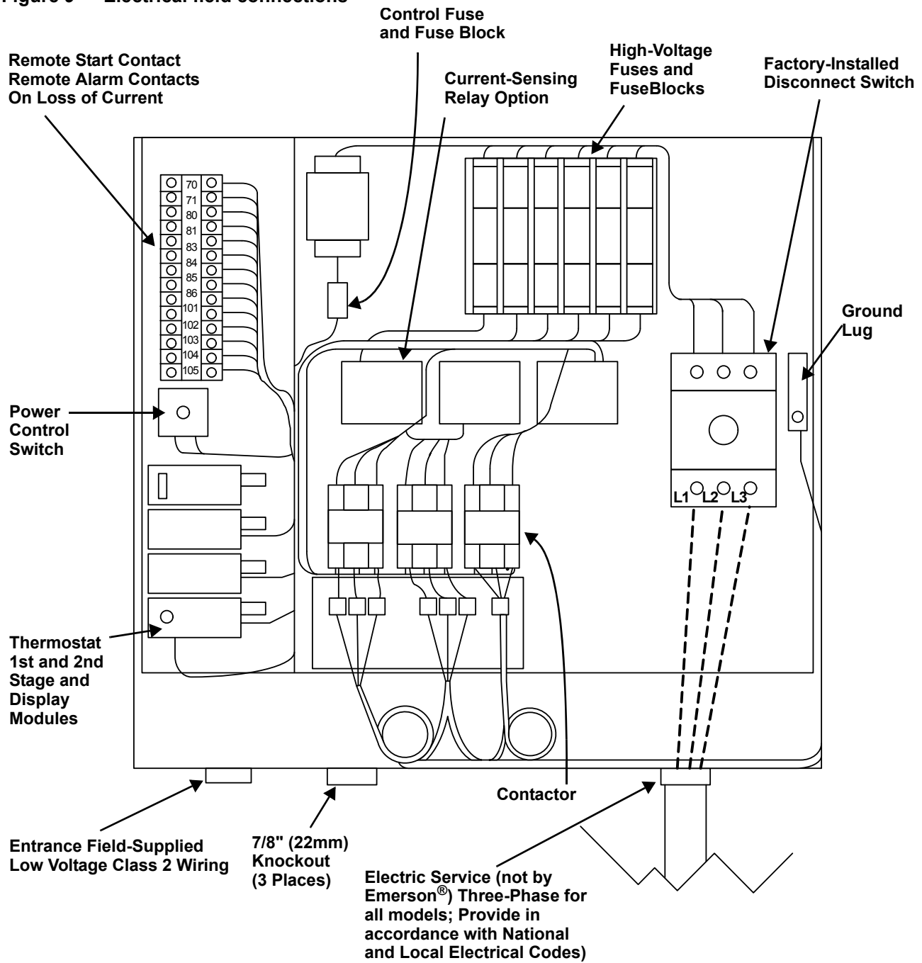
Figure 9 Electrical field connections
