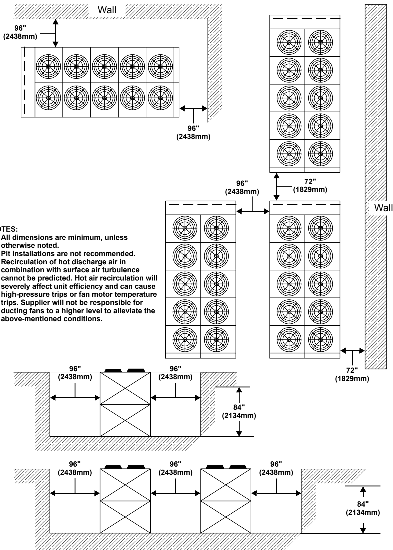
Figure 4 Clearance considerations
