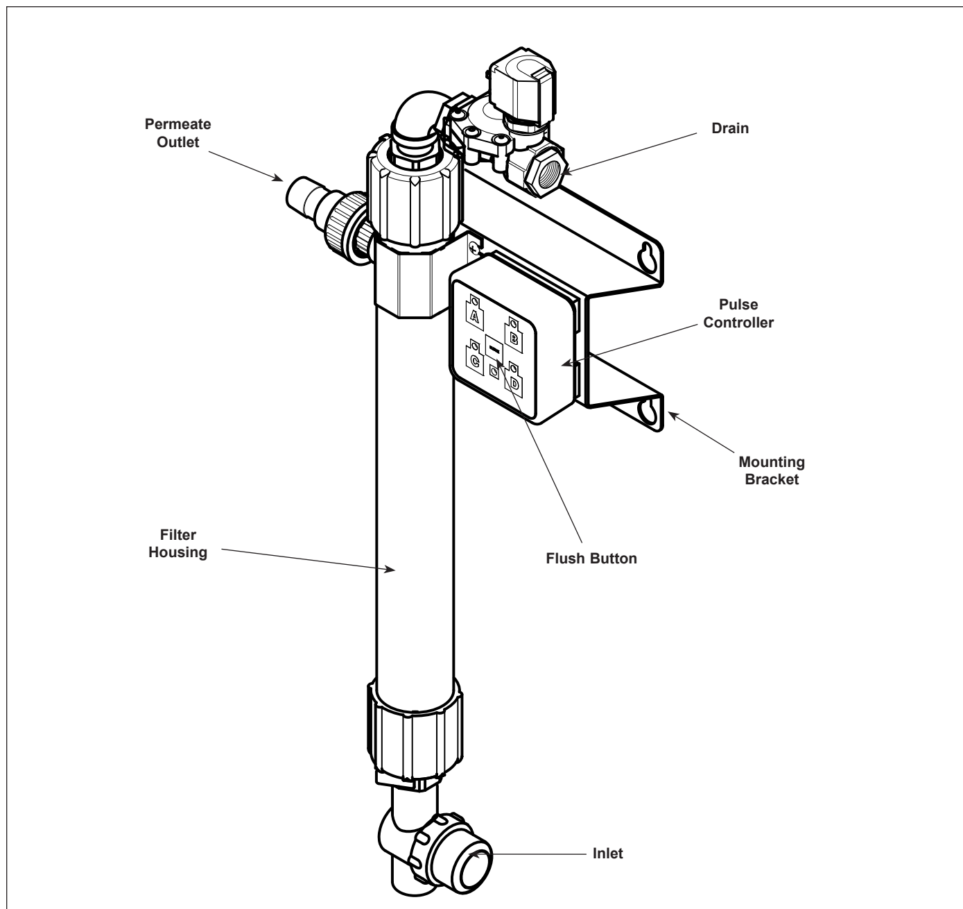
Figure 1. Components
