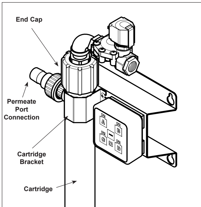
Figure 4. Replacing the Ultra Filter Cartridge
