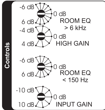
Figure 6: Control panel
