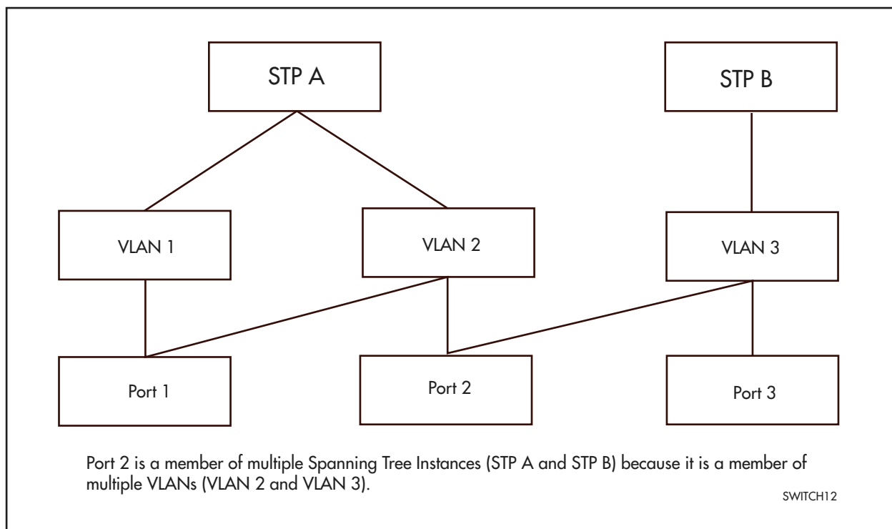
Figure 19: Port membership of VLANs which belong to different spanning tree instances (on Rapier i Series switches only).
