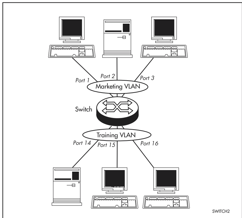
Figure 16: VLANs with untagged ports.
