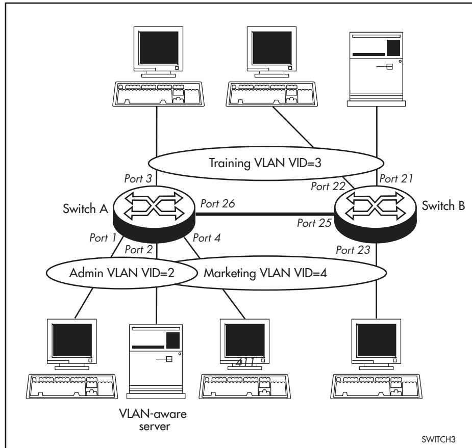
Figure 15: VLANs with tagged ports.
