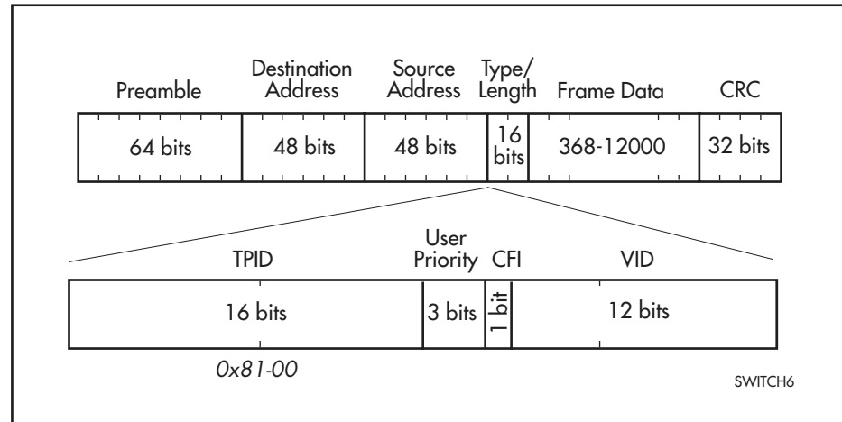
Figure 14: Format of user priority and VLAN data in an Ethernet frame.
