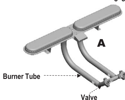
Correct burner-to-valve engagement
