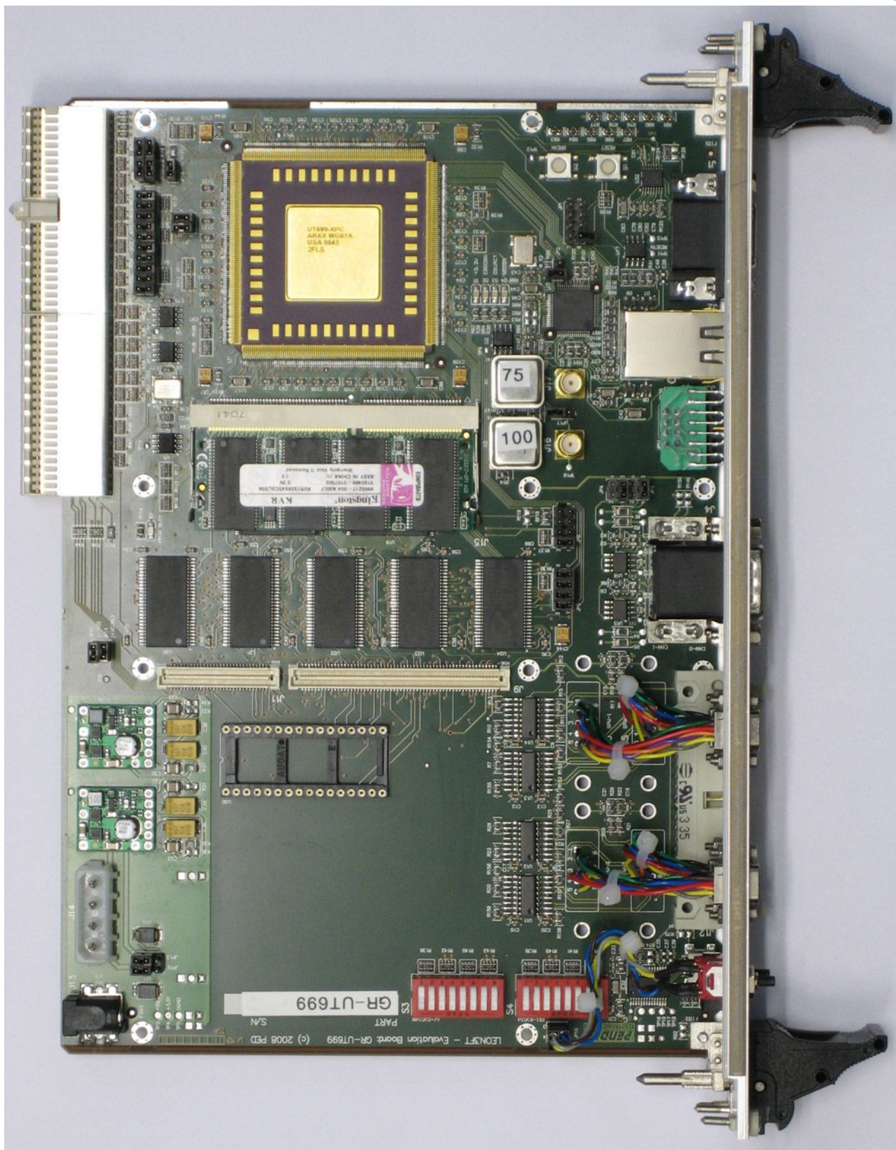
Figure 4-3: GR-UT699 Assembly Photo
