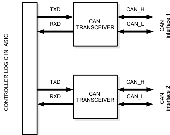
Figure 2-4: Block Diagram of the CAN interface
