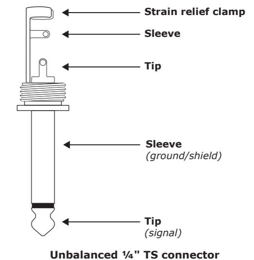
Fig. 4.3: 1/4" TS connector
