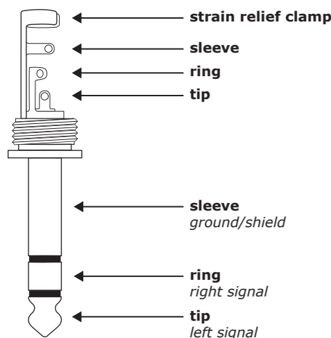
Fig. 4.4: 1/4" TRS connector
