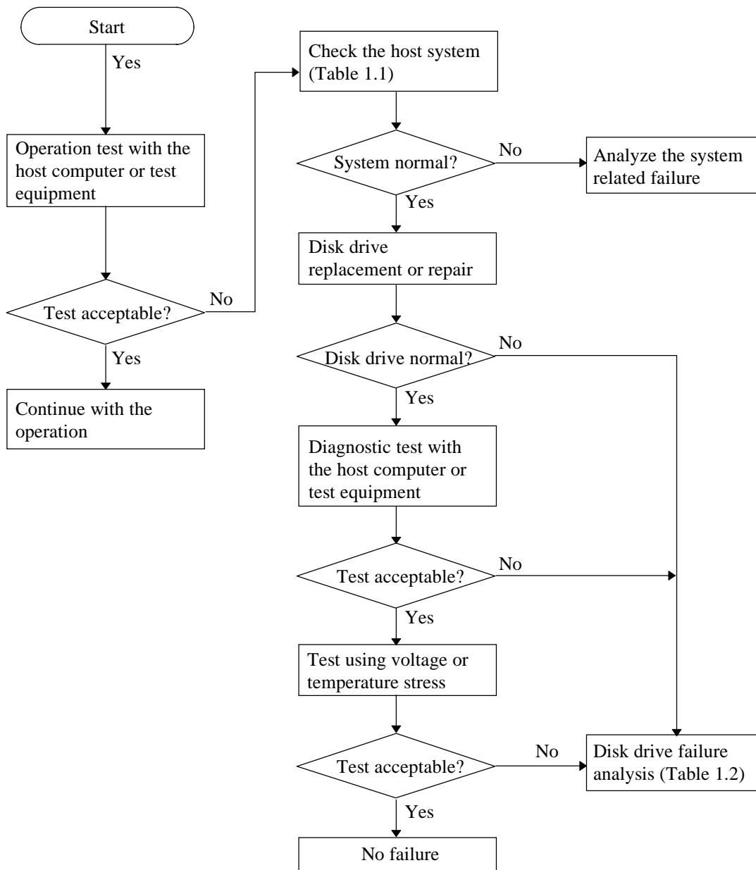
Figure 1.3 Test flowchart
