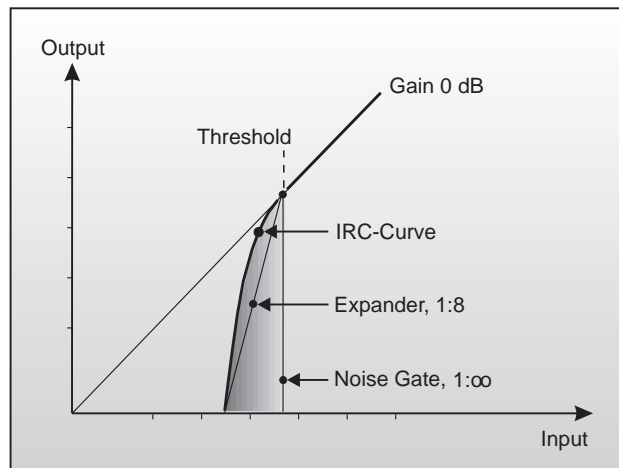
Fig. 5.1: IRC curve characteristic of the Expander
