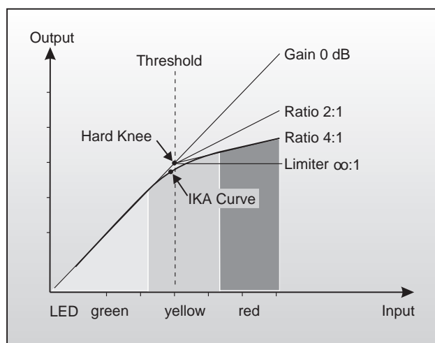
Fig. 5.2: IKA characteristic of the Compressor section
