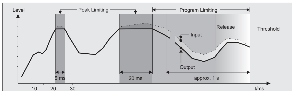
Fig. 5.3: IGC characteristic of the Limiter section
