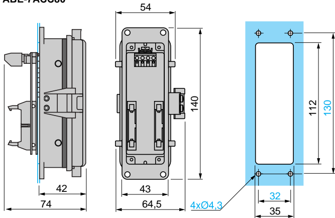
ABE-7ACC80
