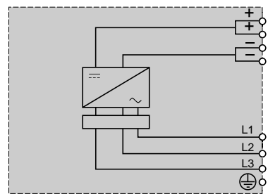
ABL-7UP●●●●●
