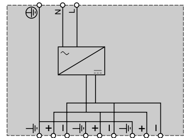
ABL-7RP2410
