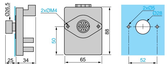
ABE-7ACC82, ABE-7ACC83
