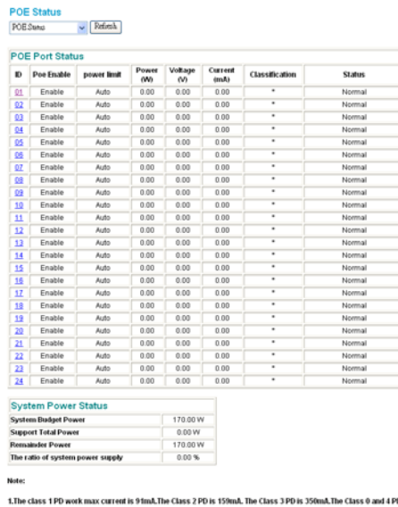
Figure 32. PoE Status
