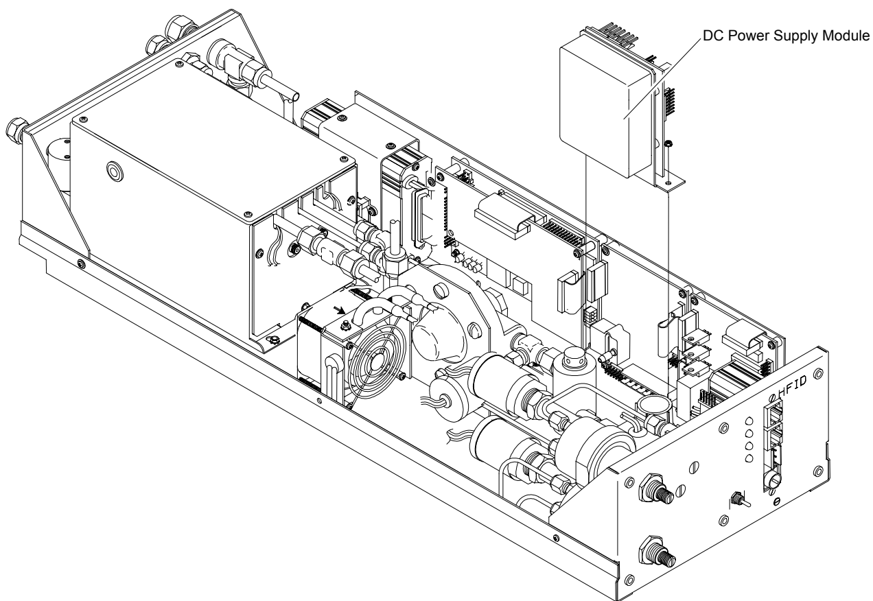
Figure 4-19. DC Power Supply Module Replacement
