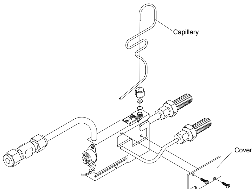
Figure 4-10. Thermal Block Assembly
