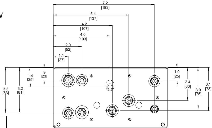
Figure 2-5. HFID Outline and Mounting Dimensions
