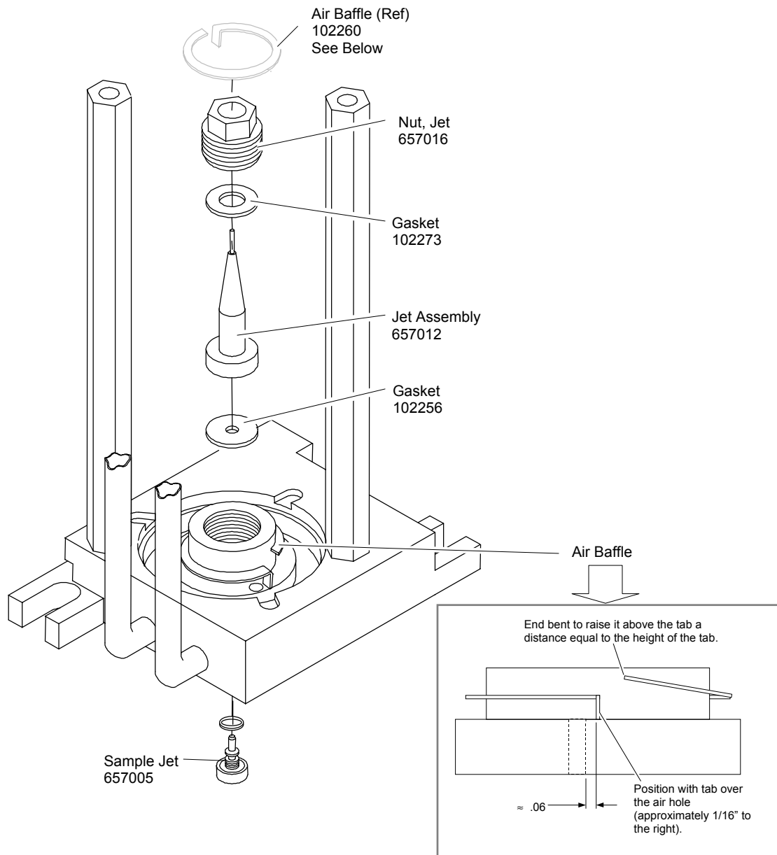
Figure 4-8. Burner Jets
