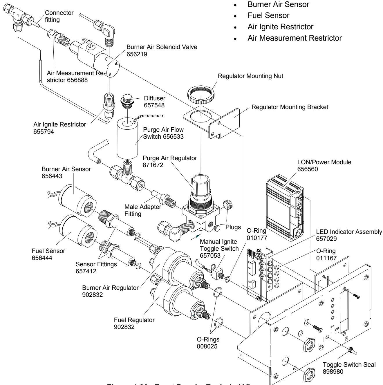
Figure 4-20. Front Panel – Exploded View
