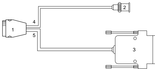
Test Cable Connections
