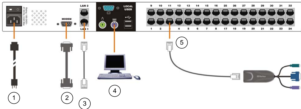
Figure 6 Back Panel of Dominion KX
