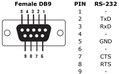
RS-232 Pin Assignment Diagram
