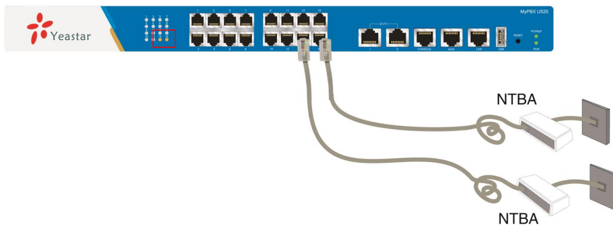
Figure 3-6 Connection of BRI ports
