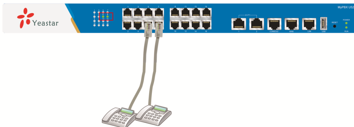
Figure 3-7 Connection of FXS ports
