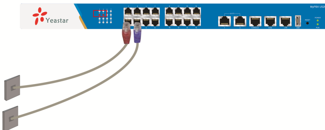
Figure 3-3 Connection of FXO ports
