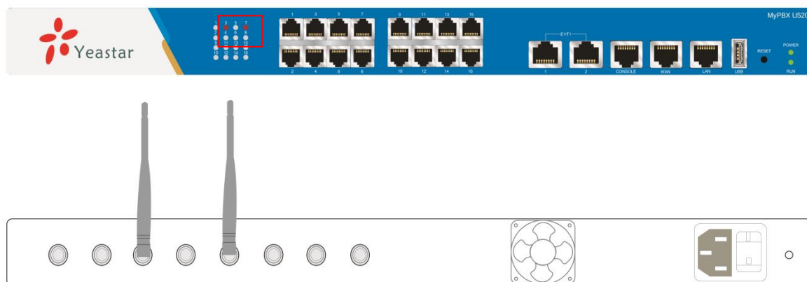
Figure 3-5 Connection of GSM/UMTS ports
