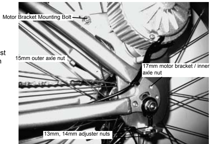
4 Motor Bracket Mounting Bolts
