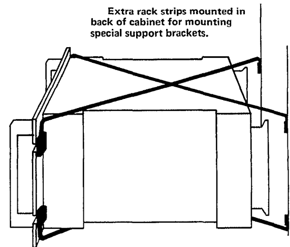
P-2200 mounted in rack showing support brackets made from bent pieces of 1/8" steel rod with nuts welded to their ends.
