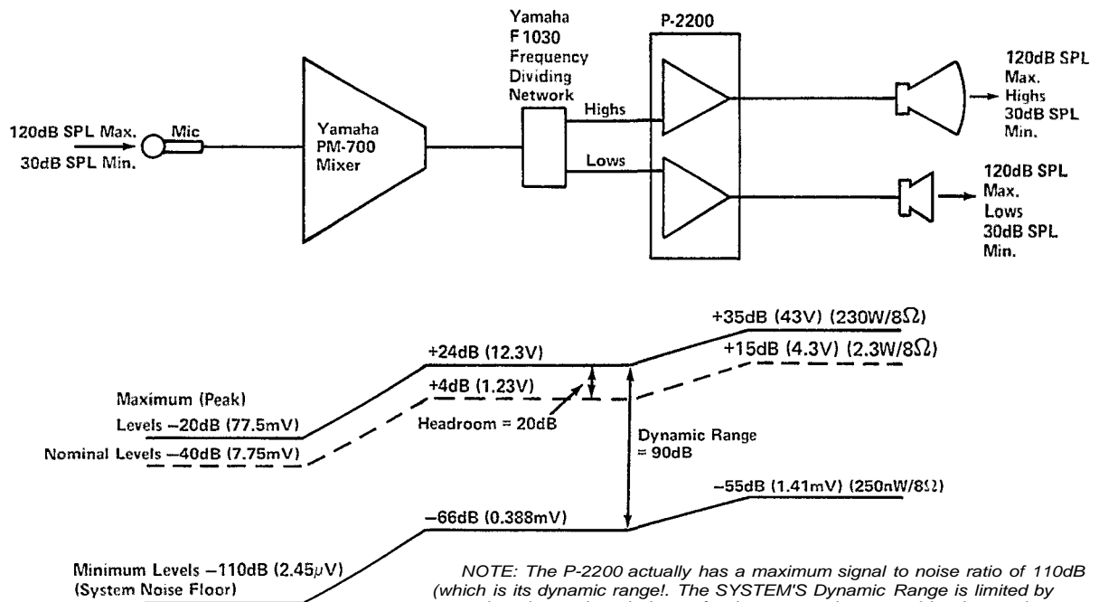
Fig. 33 - Dynamic Range in an Audio System
