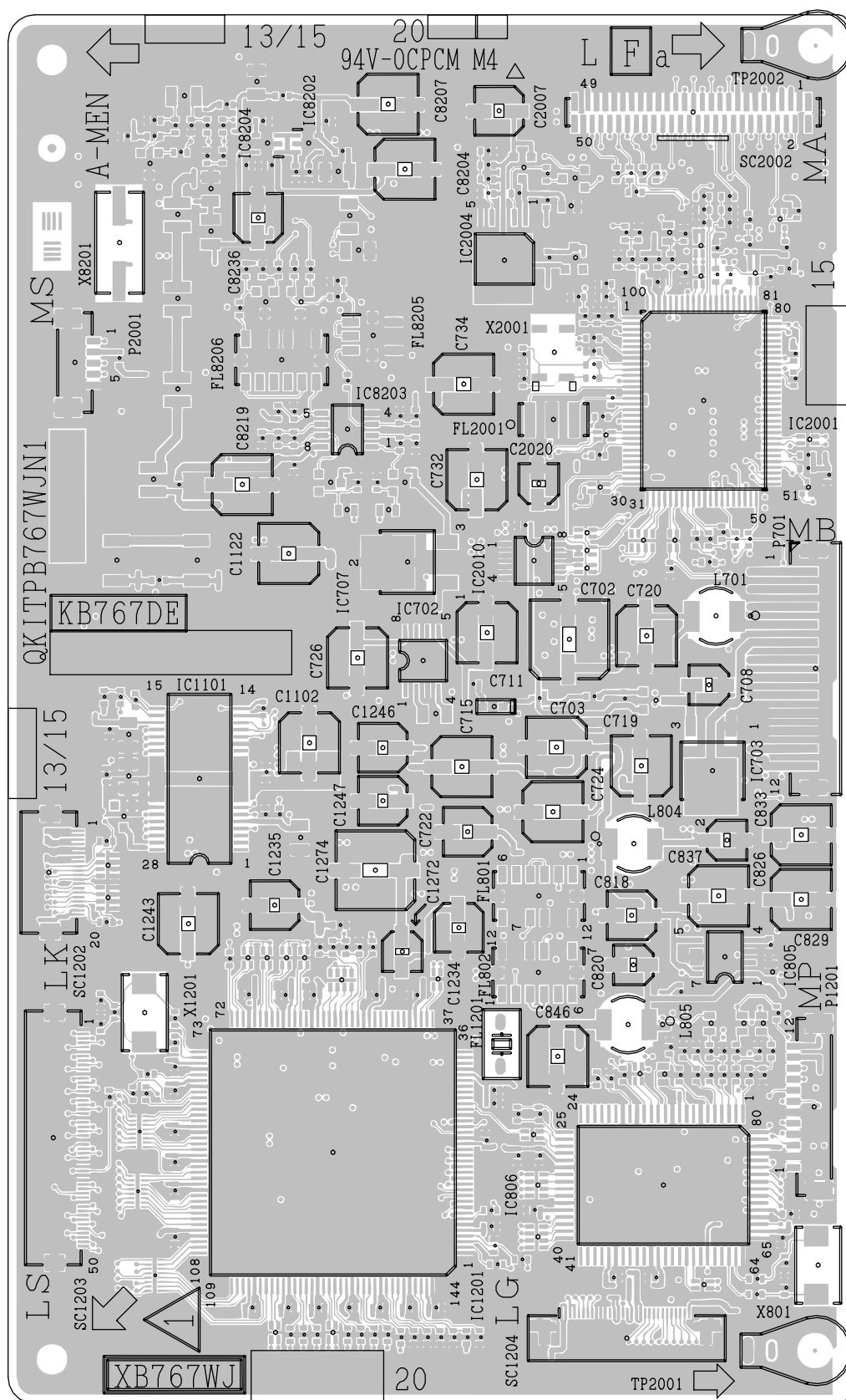
MAIN Unit (Side-A)
