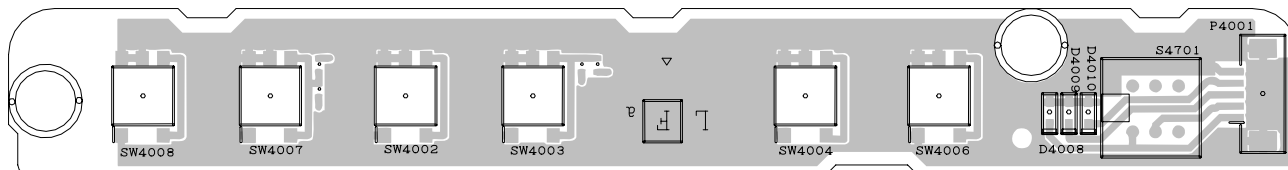
OPERATION Unit (Side-A) (QPWBSB770WJN2)
