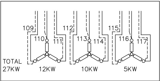
Y CONNECTION 380/415V ONLY
