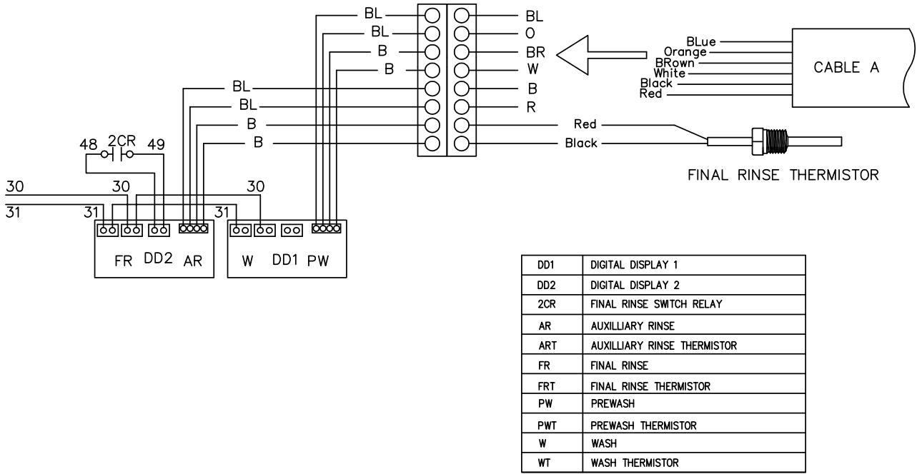
CONTROL CABINET CONNECTIONS
