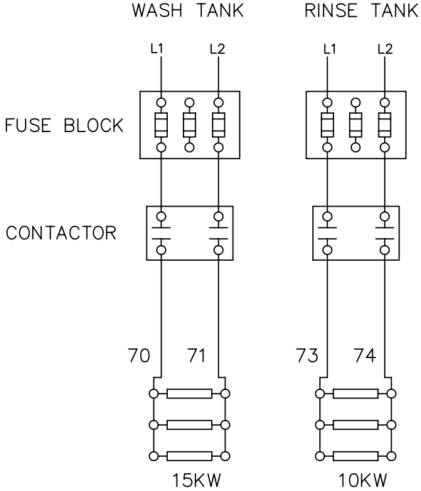
1 PHASE CONNECTION
