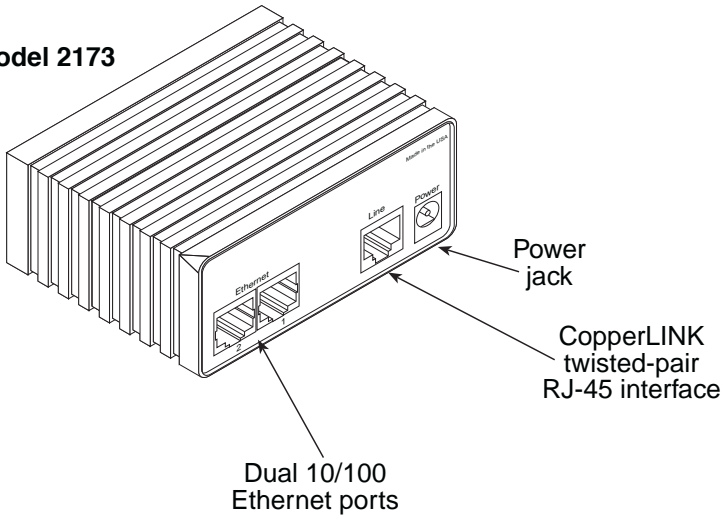
Figure 2. Model 2173 standalone rear panel
