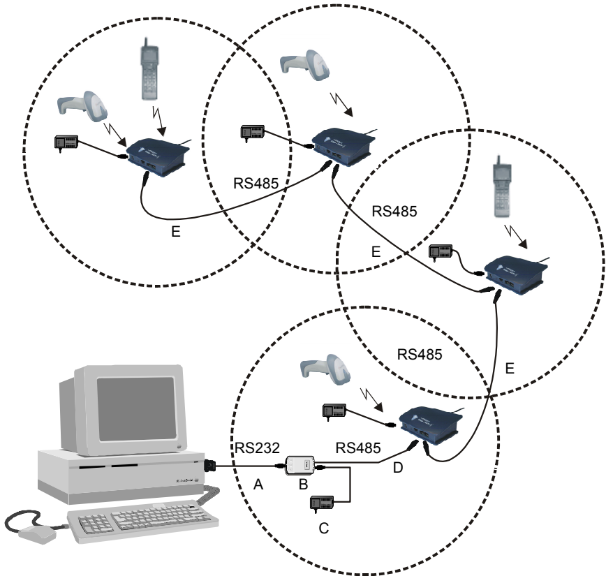
Figure 8 - RS485 connection
