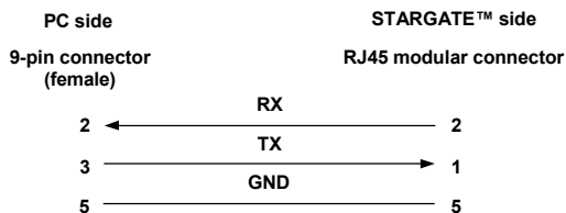
Figure 7 - RS232 pinout
