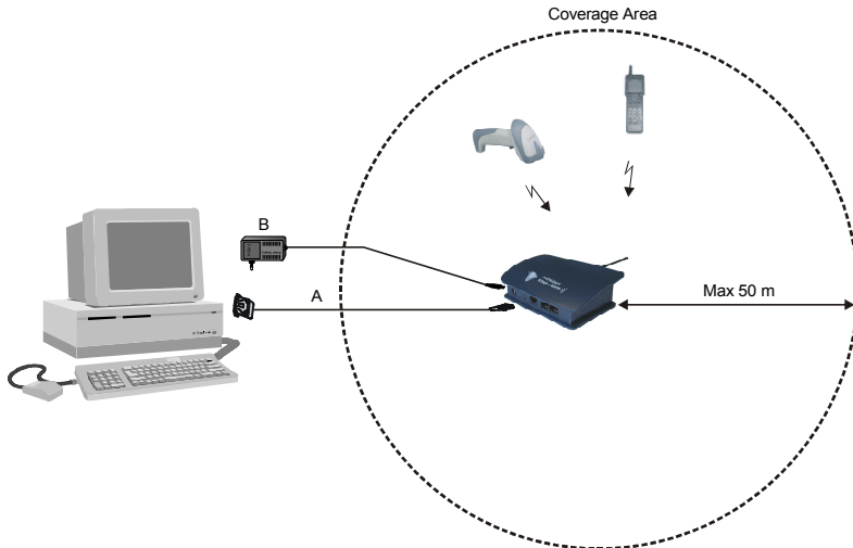
Figure 4 - RS232 connection
