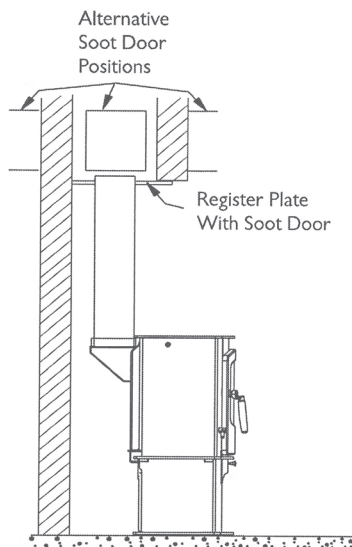
Fig 11: Horizontal register plate with optional vertical rear flue connection.
