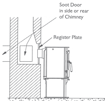
Fig 8: Vertical register plate with bricked up fireplace.
