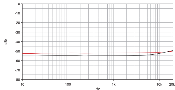
Figure 7.7 Common mode rejection ratio vs. frequency (Measurement of a typical performance of Ch 1 & Ch 2)
