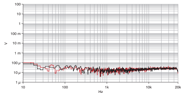
Figure 7.8 FFT of noise level (no input signal applied, analog input, 32 dB amplifier gain) (Measurement of a typical performance of Ch 1 & Ch 2)
