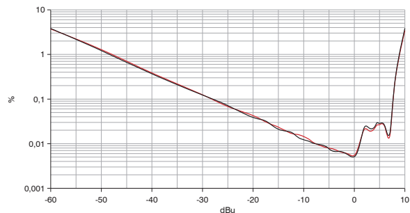
Figure 7.6 DIM100 vs. input level (32 dB amplifier gain) (Measurement of a typical performance of Ch 1 & Ch 2)
