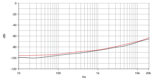
Figure 7.5 Channel separation vs. frequency @ 120 W/4 \Omega (Measurement of a typical performance of Ch 1 \rightarrow Ch 2 & Ch 2 \rightarrow Ch 1)
