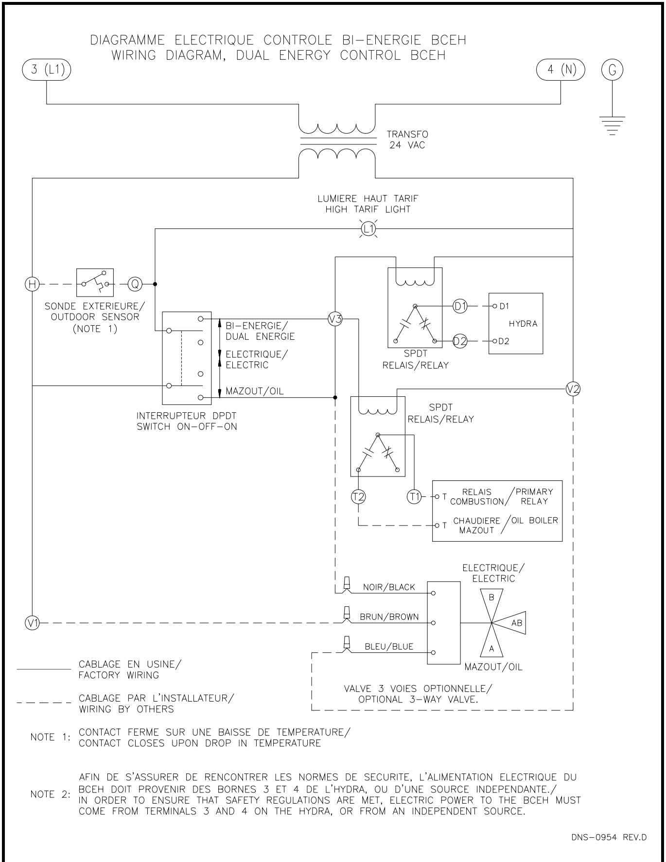
FIGURE 6 Ladder Diagram
