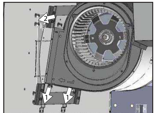
12. Position blower inside insert body as shown by: 1) Rest the bottom horizontal ducting bracket on the two support clips located on the interior back wall of the insert. 2) Pivot top horizontal ducting bracket to meet captive nuts on interior back wall.
