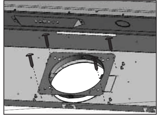
10. (Round Ducting) From inside the insert, push 8" round adaptor through the back knock-out and secure to interior back wall of insert with (4) M4 x 6mm screws.
