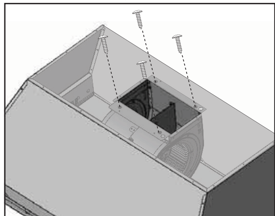
6. Remove blower from insert by removing the (4) 3/16" x 3/8" screws from the top of the insert. Set screws aside for later usage.
