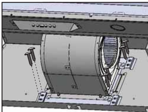
13. Secure blower to captive nuts on interior back wall of insert with (8) 3/16" x 3/8" screws, (4) screws for each bracket. Seal any gaps around the knock-out plate by using certified aluminum duct tape. Plug in blower moxex plug.
