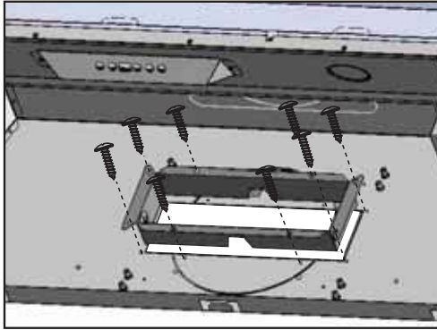
10. (Rectangular Ducting) From inside the insert, push 3-1/4" x 10" rectangular adaptor through the back knock-out and secure to interior back wall of insert with (8) M4 x 6mm screws.
