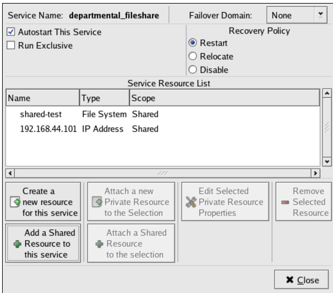
Figure 5.9. Adding a Cluster Service
