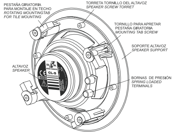
Fig. 2 –CL-5, back view
