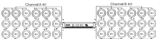
Fig. 4.1 – Series-parallel connection of a large number of speakers per channel
