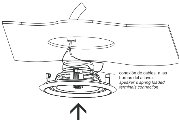
Fig. 8 – terminal connection; speaker positioning
