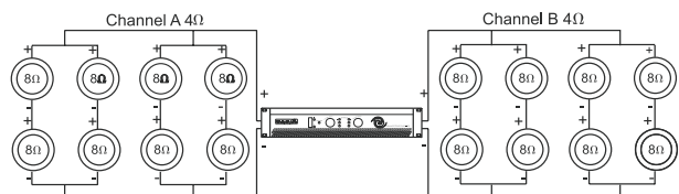
Fig. 4 - series-parallel connection
