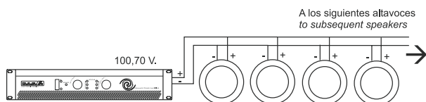
Fig. 5 – Parallel connection of transformer units
