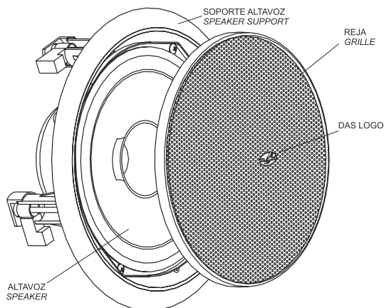
Fig. 1 –CL-5, front view
