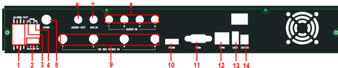
Fig 2-5 Rear Panel for 4-ch
