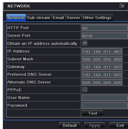
Fig 4-26 Network Configuration-Network
