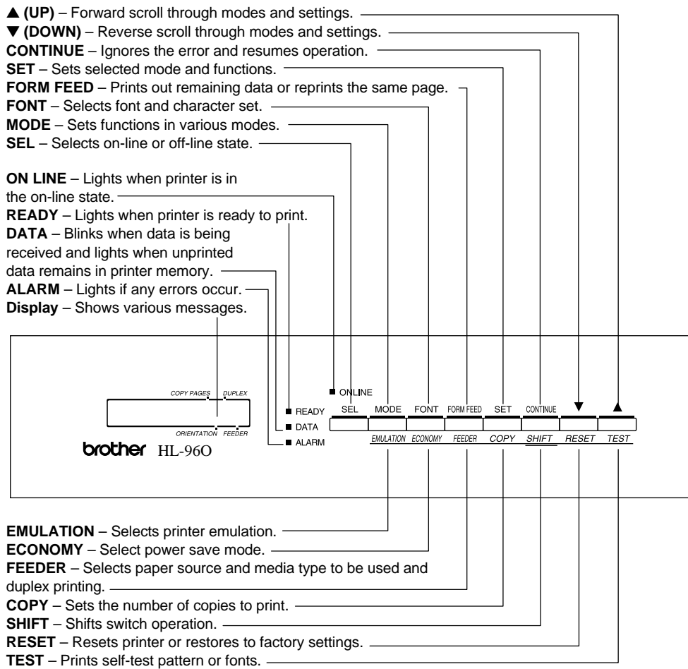
Fig. 3-2 Switch Operation in NORMAL and SHIFT Modes
