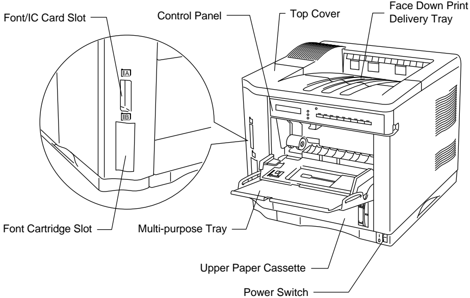
Fig. 2-3 Front View
