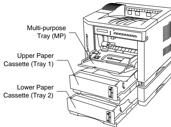
Fig. 3-5 Cassette Feed
