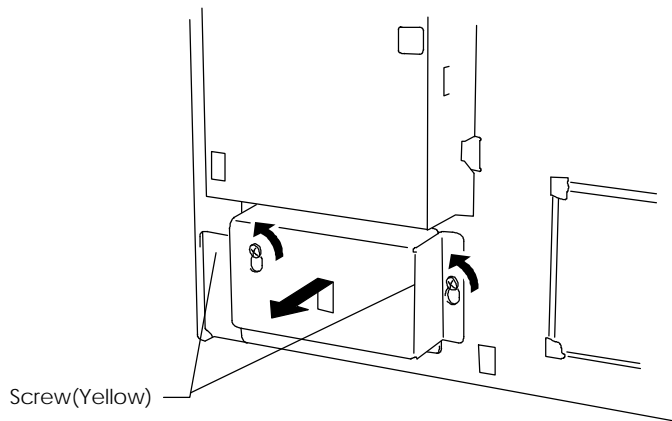
Fig. 5-6 Removing the Metal Cover
