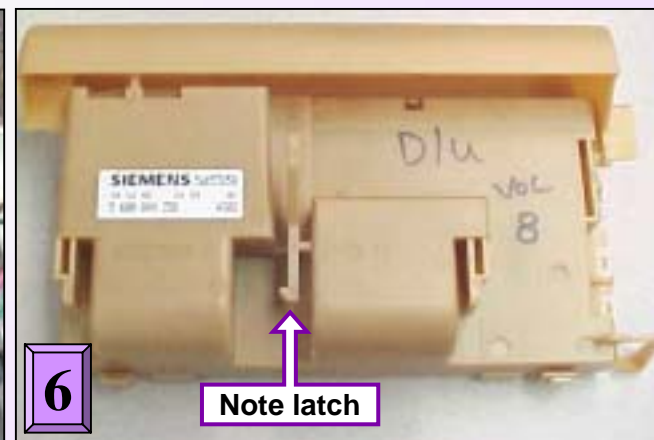
6 Align module tabs when reassembling
