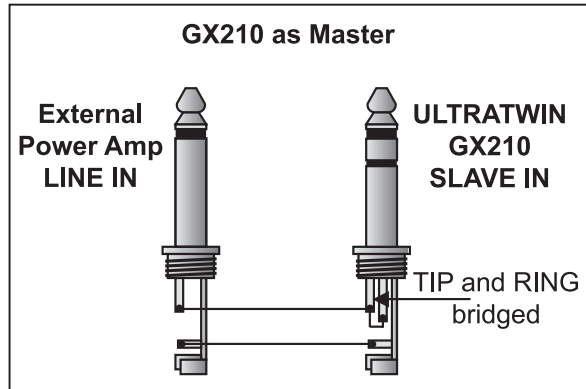
Fig. 2.3: The ULTRATWIN GX210 as master
