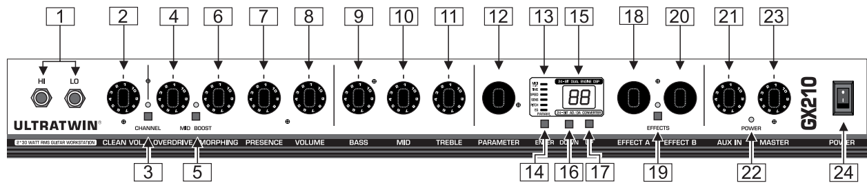
Fig. 1.2: The front panel control elements
