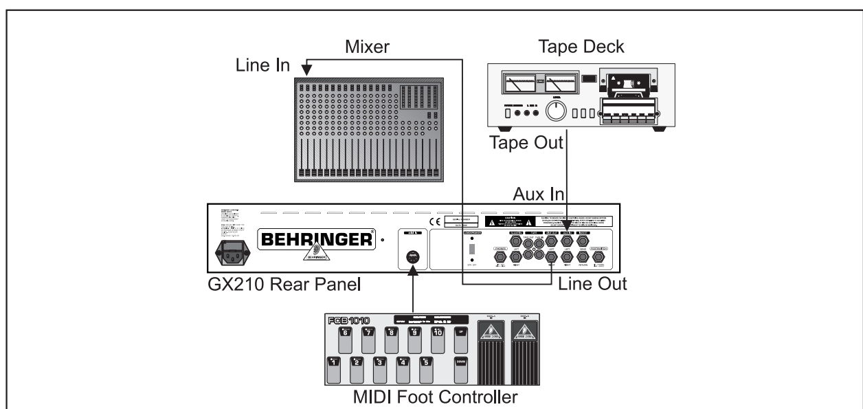
Fig. 2.2: Expanded setup
