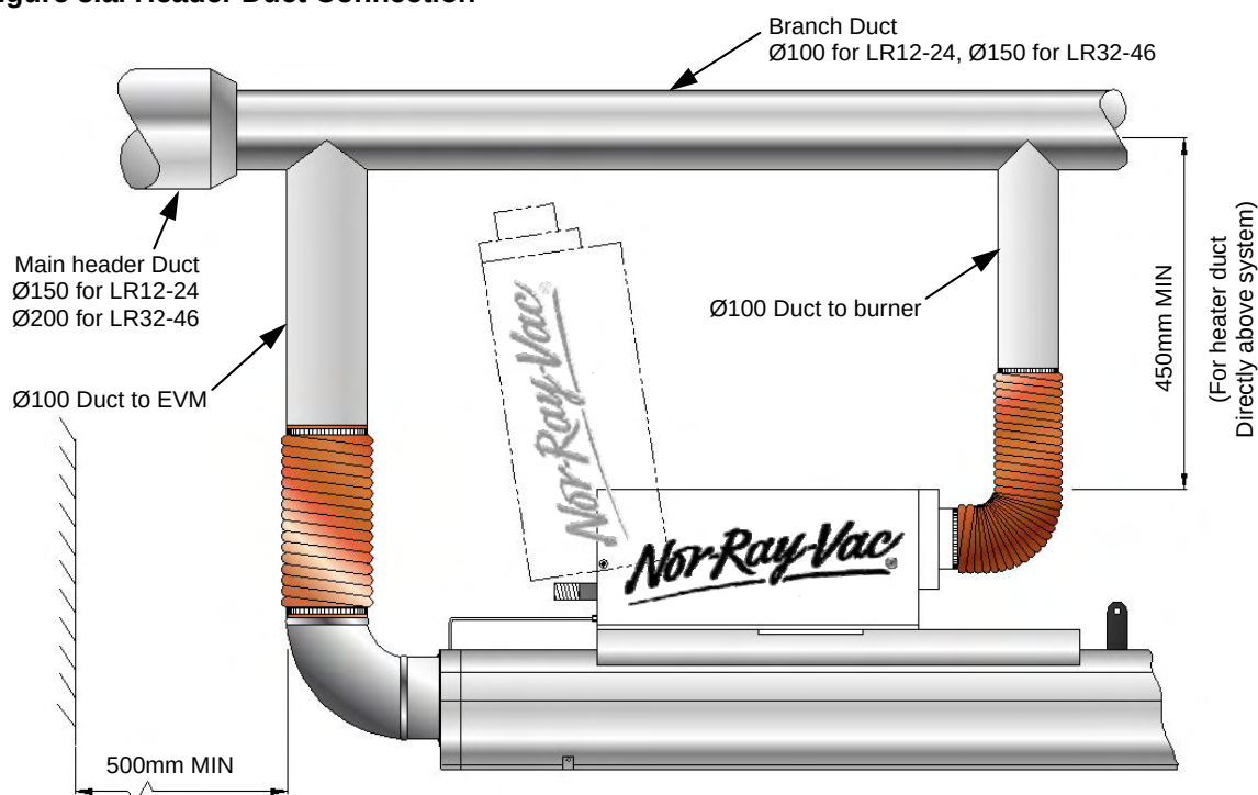
Figure 5.a. Header Duct Connection
