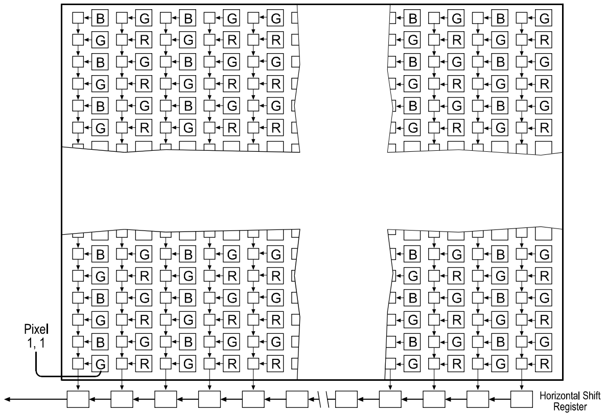
Figure 3-15: Bayer Filter Pattern on the A202kc
