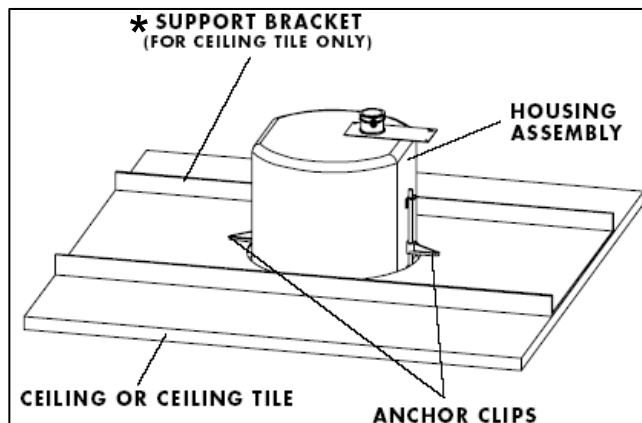
Figure 6: Flush Mount Enclosure in the Ceiling
