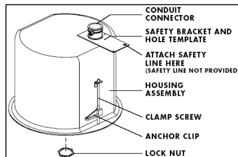
Figure 2: Plenum Rated Back Can Assembly
