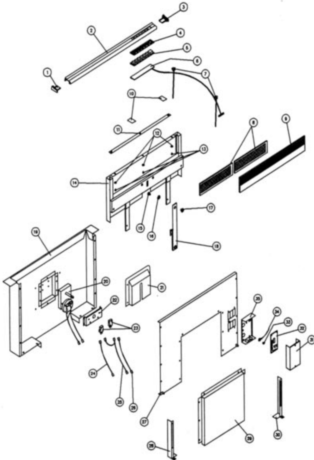
RAISED VENT WITH REMOTE BLOWER - MODELS: RVR30 / RVR36 / RVR46
