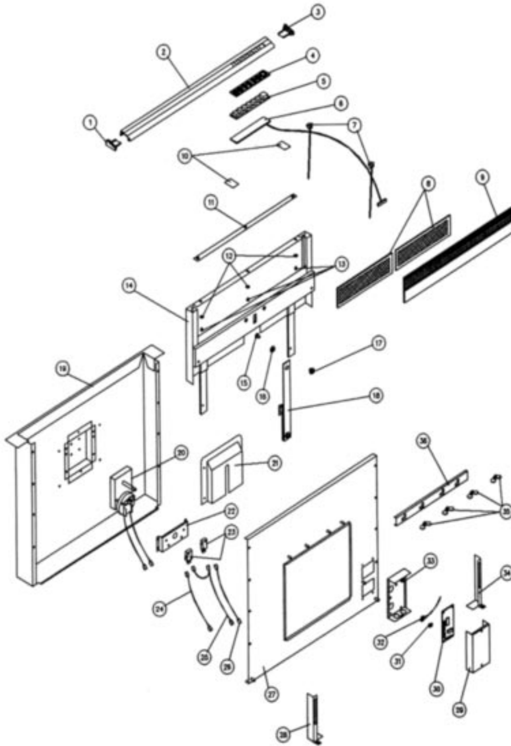
RAISED VENT WITH CABINET BLOWER - MODELS: RVC30 / RVC36 / RVC46
