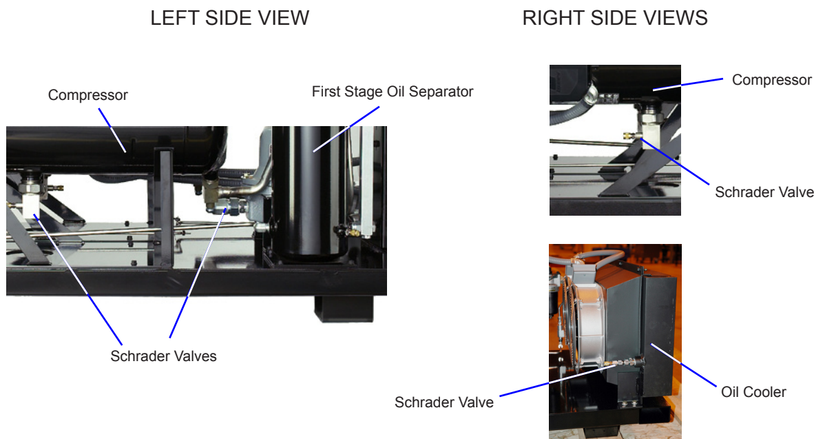
Figure 15 Adding or Draining Oil
