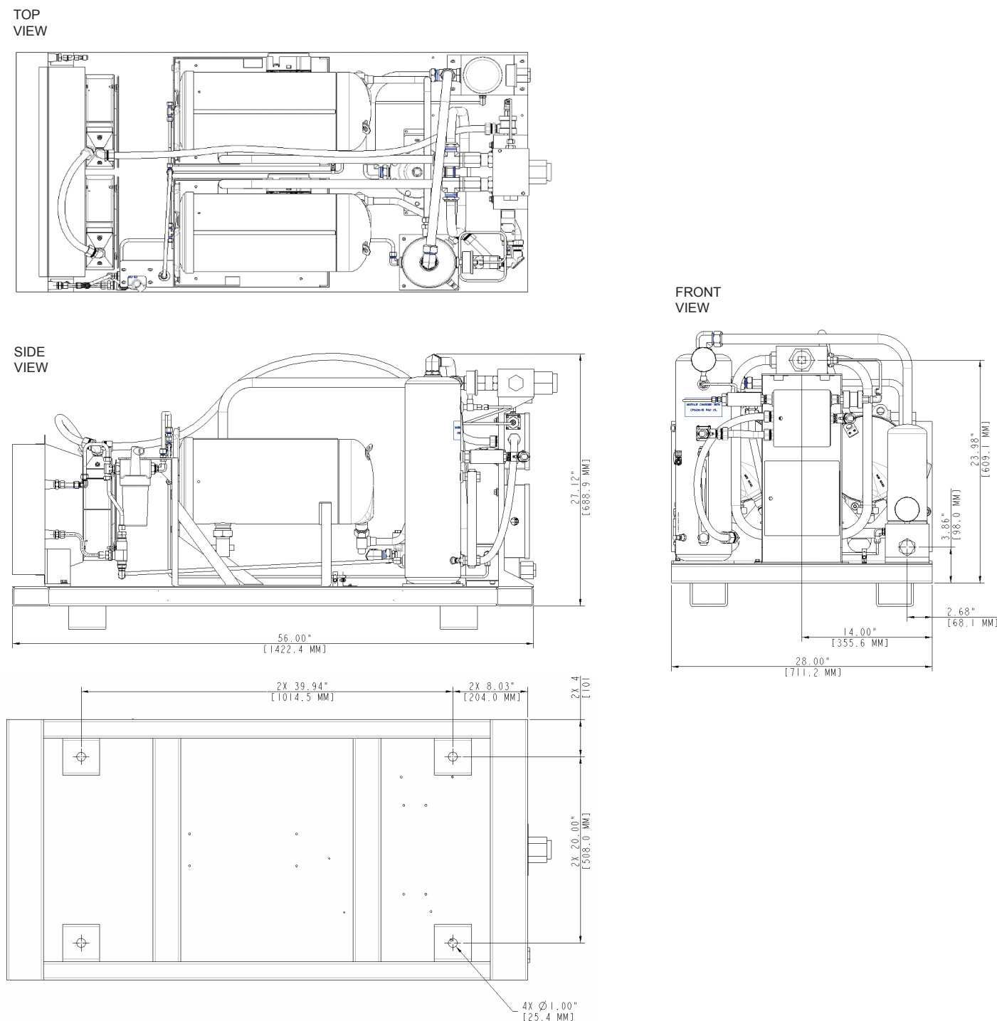
Figure 4 Compressor Module Dimensions, in. (mm)
