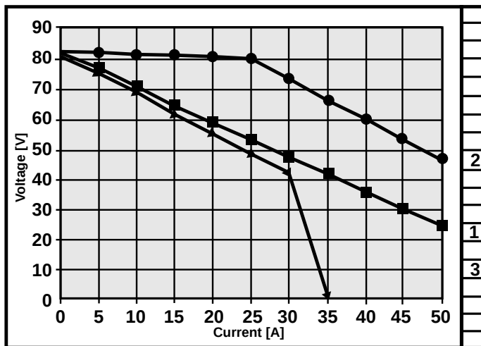
Figure 13. Current-voltage characteristic of different power supply topologies.
