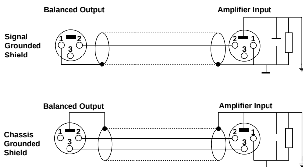
Figure 6. Balanced line
