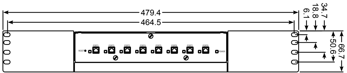
Figure 13: Rack Mount Dimensions
