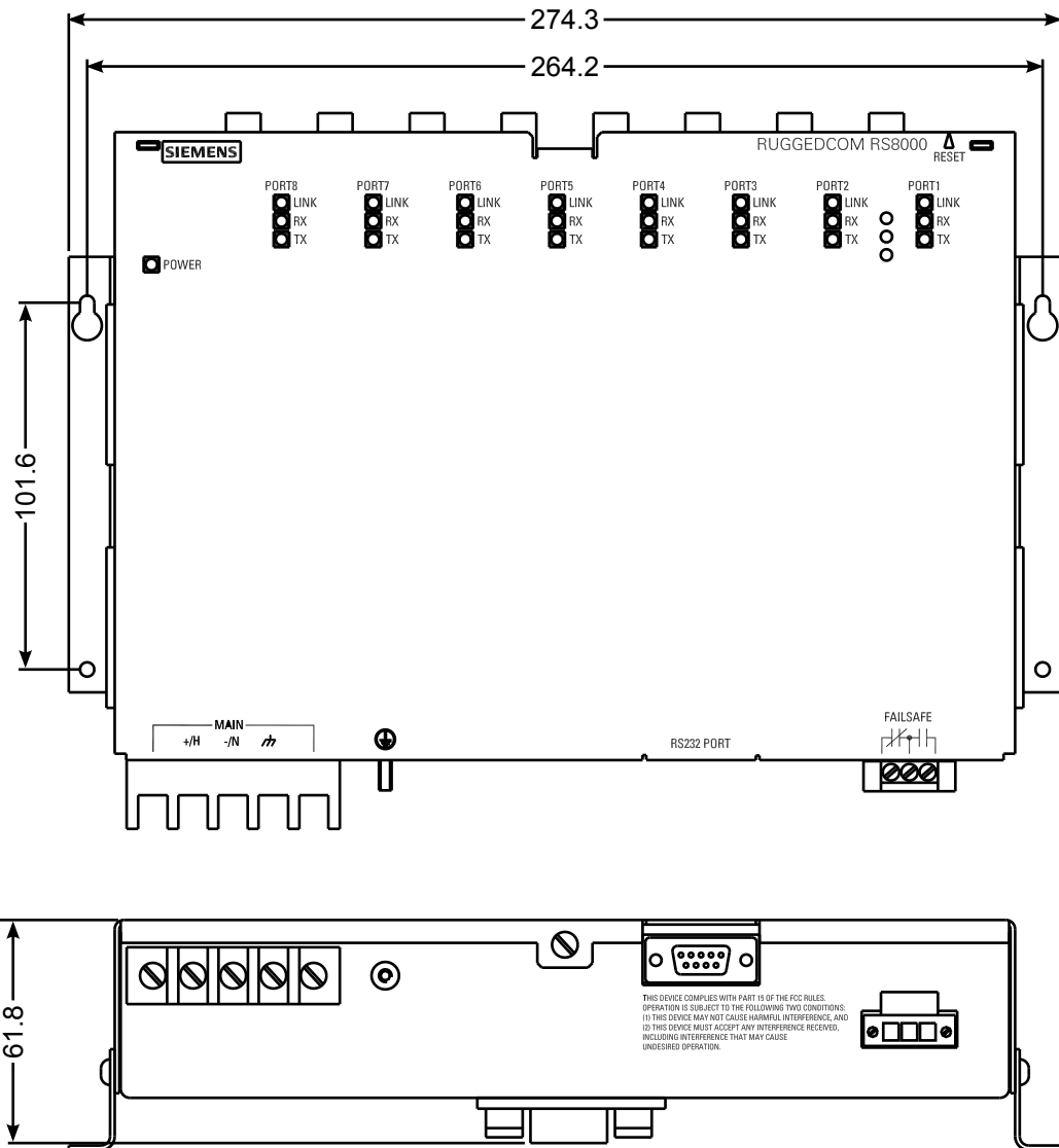
Figure 14: Panel and Din Rail Mount Dimensions
