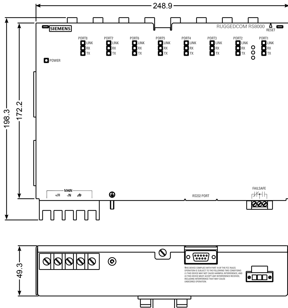
Figure 12: Overall Dimensions
