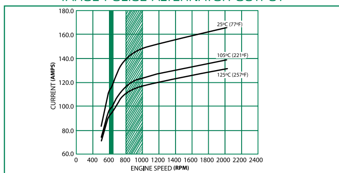
TAHOE POLICE ALTERNATOR OUTPUT
