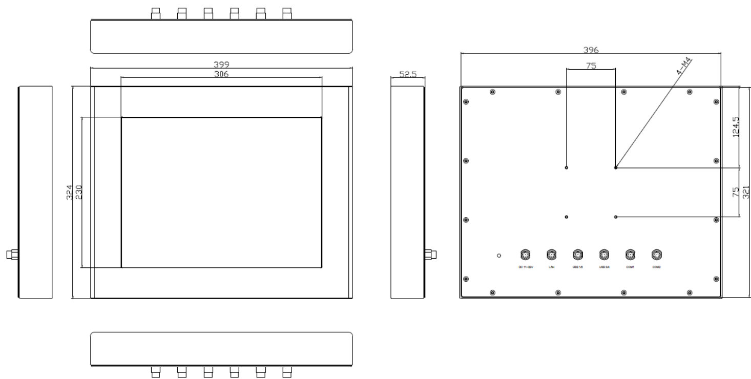
Figure 1.1: Dimensions of APC-3597B
