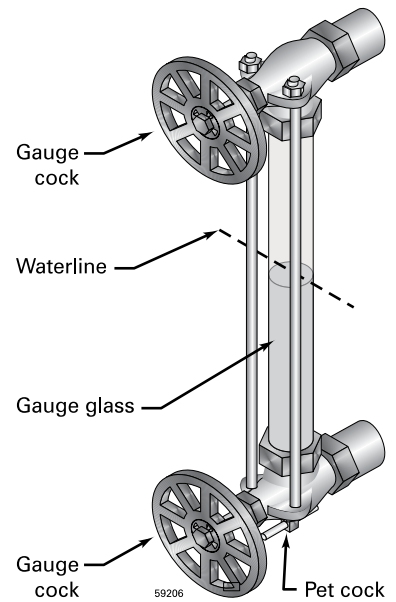
Figure 9 Gauge glass
